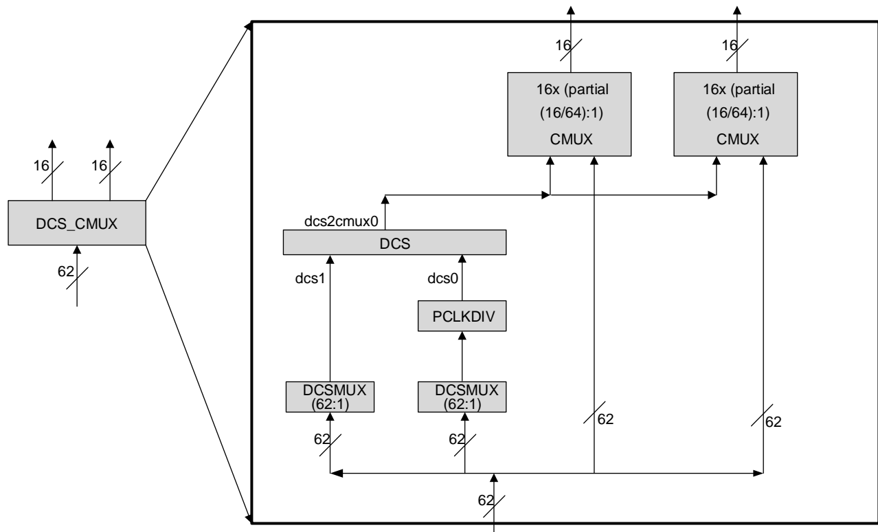
Figure 2.8. DCS_CMUX Diagram
