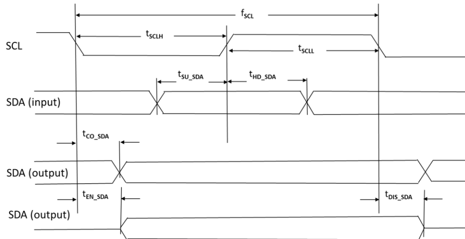
Figure 3.17. I 2 C /I3C Configuration Timing
