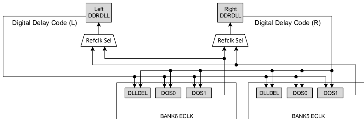
Figure 2.11. DDRDLL Architecture
