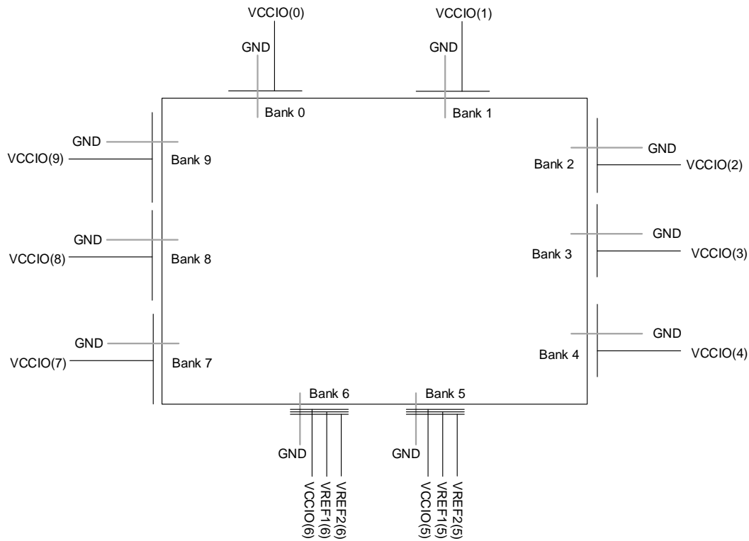
Figure 2.26. sysI/O Banking
