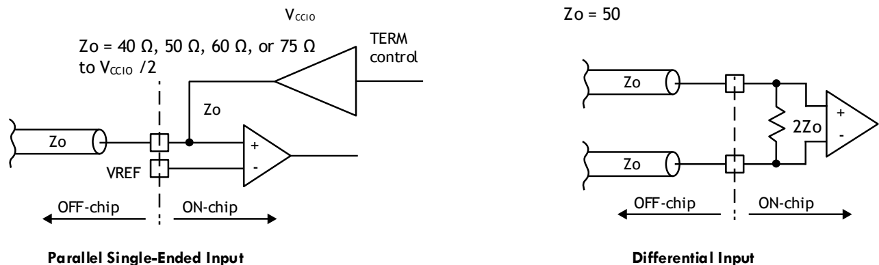
Figure 4.1. On-Chip Termination
