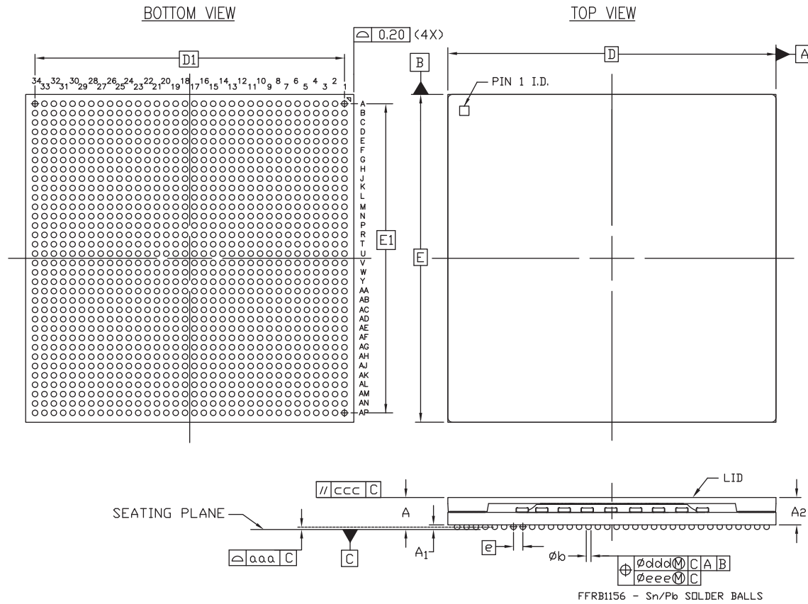
FFRB1156 - Sn/Pb SOLDER BALLS
