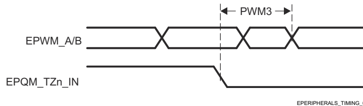
EPERIPHERALS_TIMING_05
