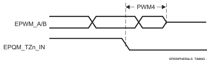
EPERIPHERALS_TIMING_06
