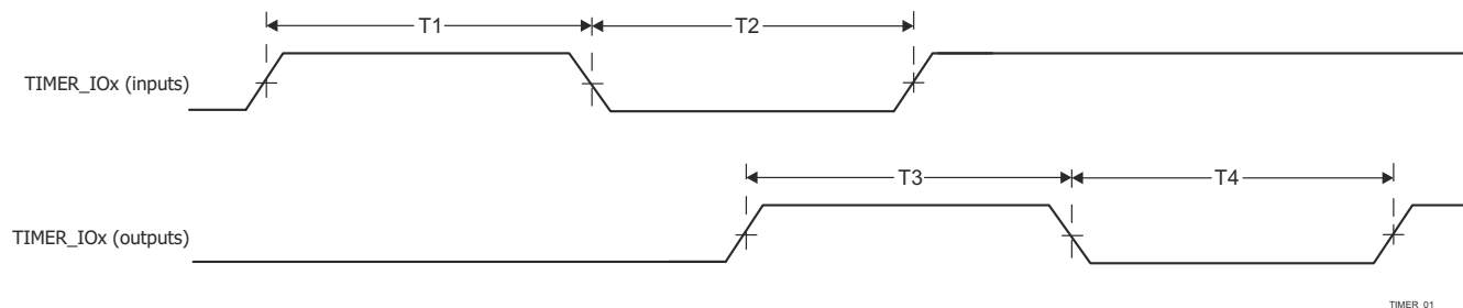
Figure 6-114. Timer Timing
