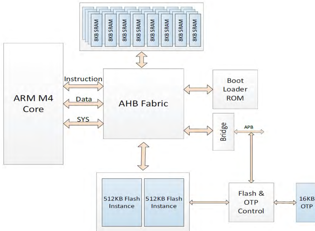
Figure 4-1: Memory Subsystem
