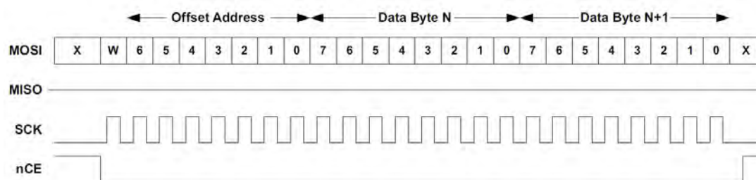
Figure 6-11: SPI White Operation
