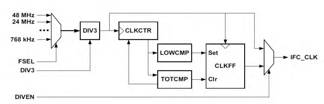
Figure 5-2: I 2 C/SPI Master Clock Generation
