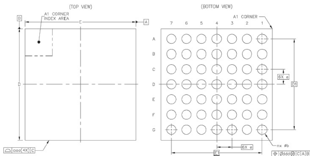
Figure 19-3: BGA Package Drawing - Notes
