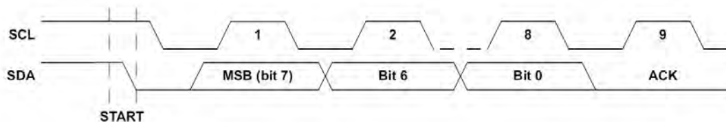
Figure 6-5: I 2 C Acknowledge
