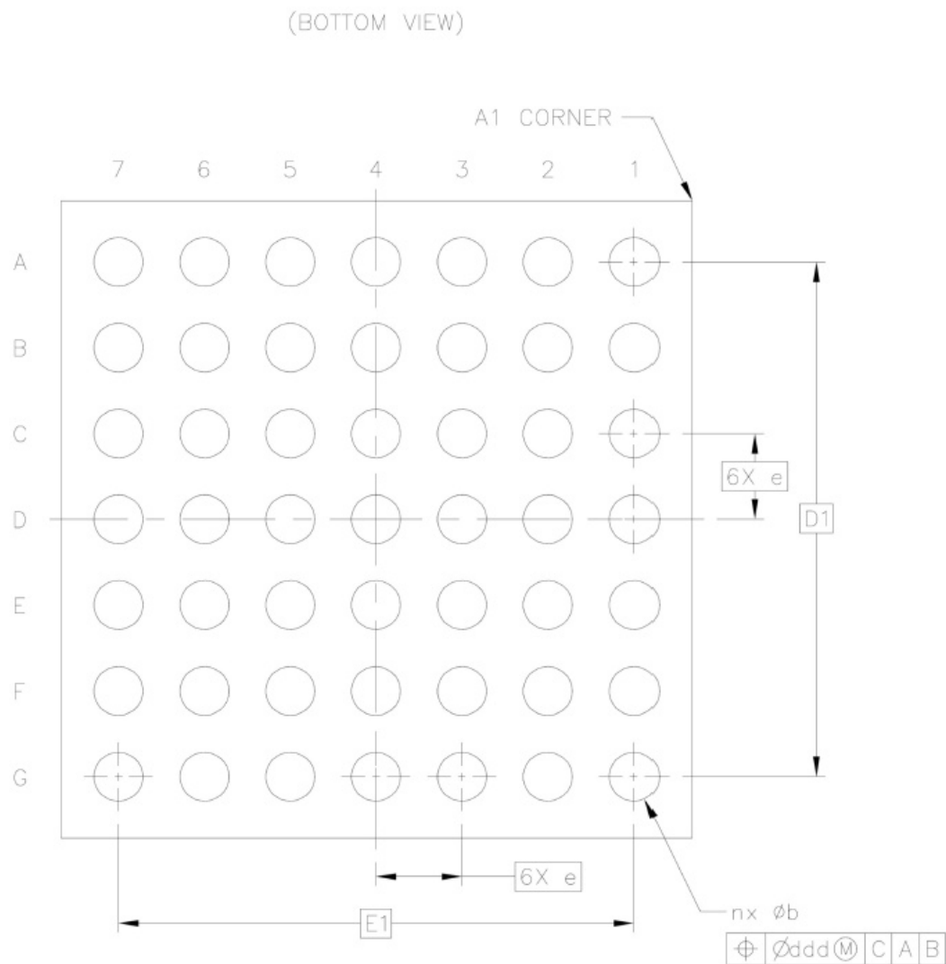
Figure 19-7: Apollo2 Thin WLCSP Drawing - Bottom View
