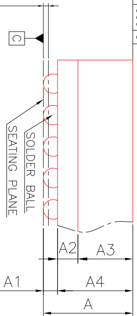
DETAIL : "A"
