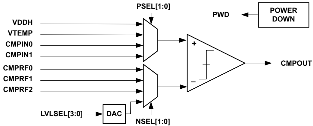
Figure 94. Block diagram for the Voltage Comparator Module
