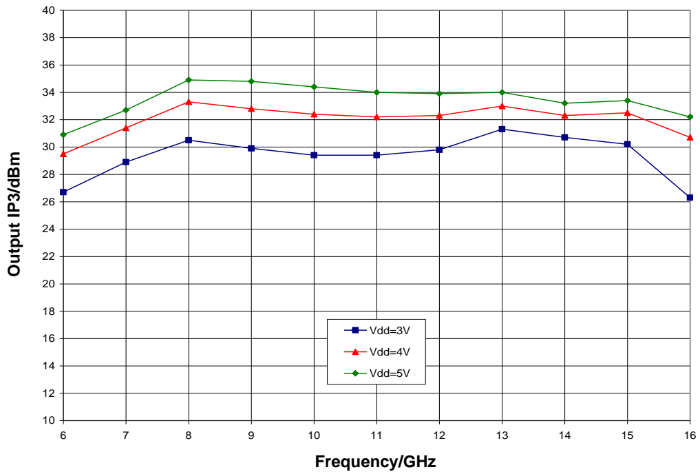
Output IP3 vs. V_{dd} , T_A = 25\text{ °C}
