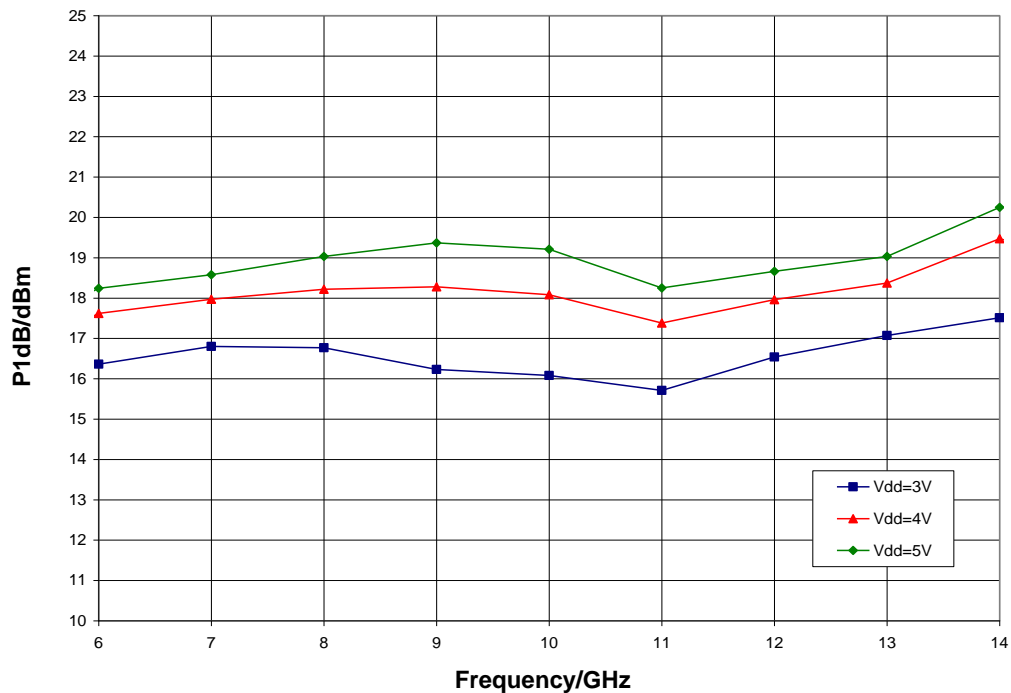
P1dB vs. V_{dd} , T_A = 25\text{ }^\circ\text{C}
