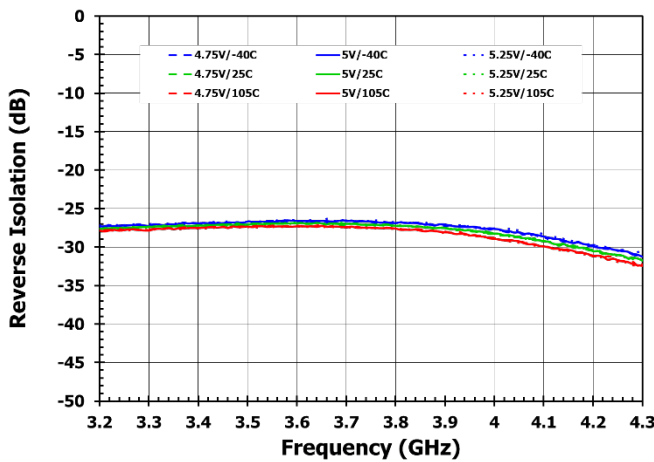
Figure 14. Reverse Isolation
