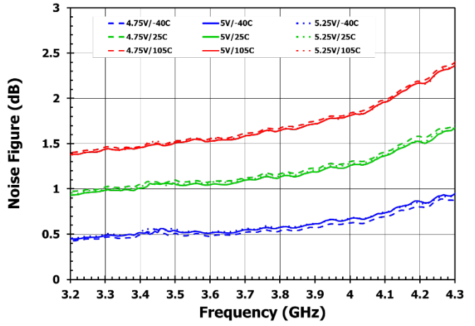
Figure 17. Noise Figure
