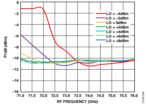
Figure 191. Input P1dB vs. RF Frequency at Various LO Powers, IF = 2000 MHz, V_{DLNA} = 4\text{ V}
