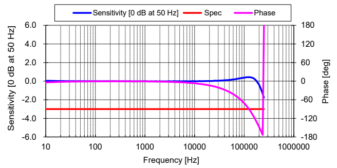
Figure 7: Frequency response
