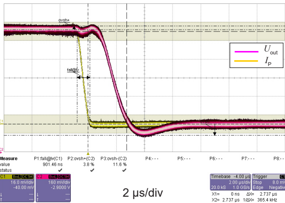
Figure 3: Step response
