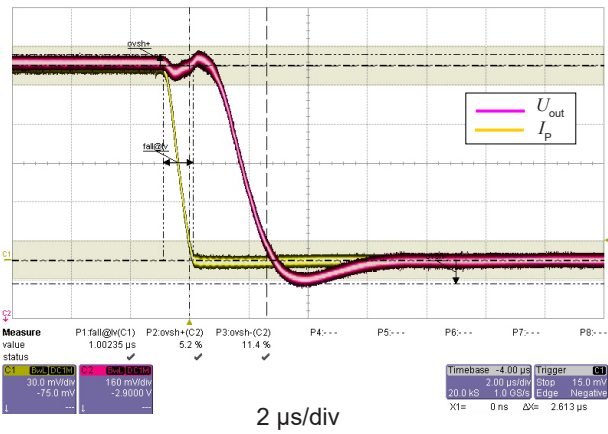
Figure 8: Step response
