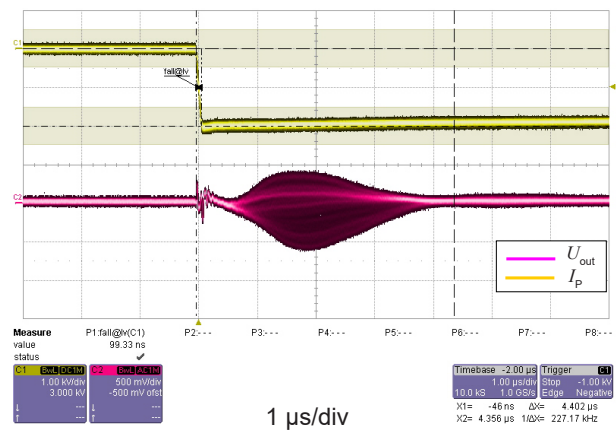
Figure 9: dv/dt
