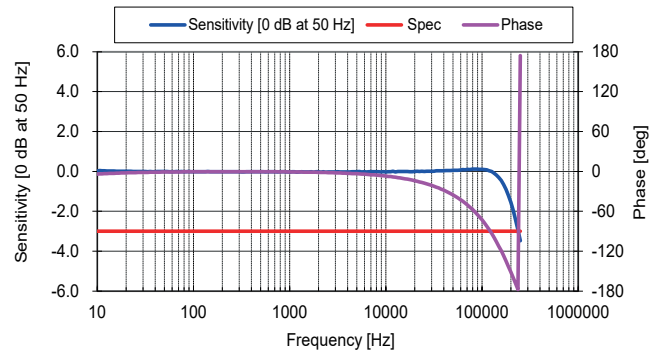
Figure 2: Frequency response
