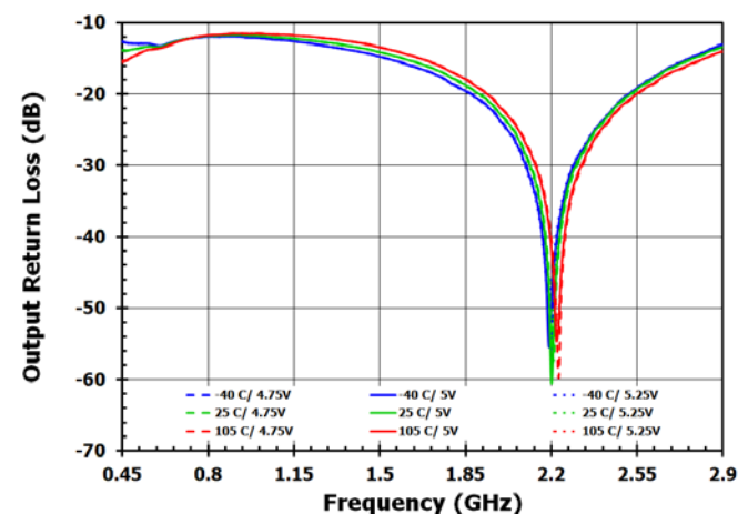
Figure 74. S22, DSA2 = 15dB, Bypass OFF
