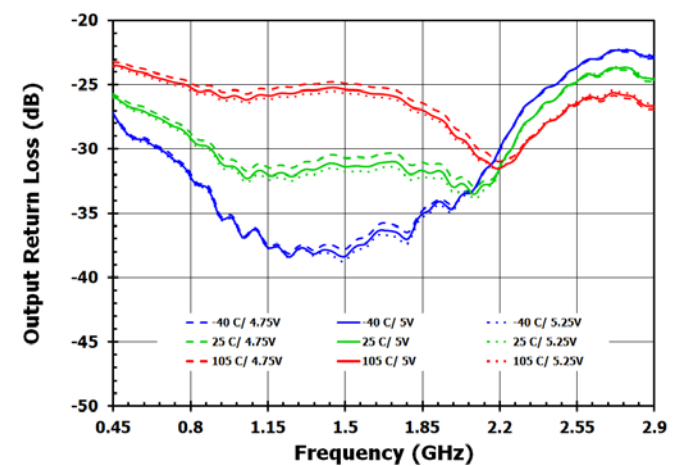
Figure 80. S22, DSA3 = 12dB, Bypass OFF
