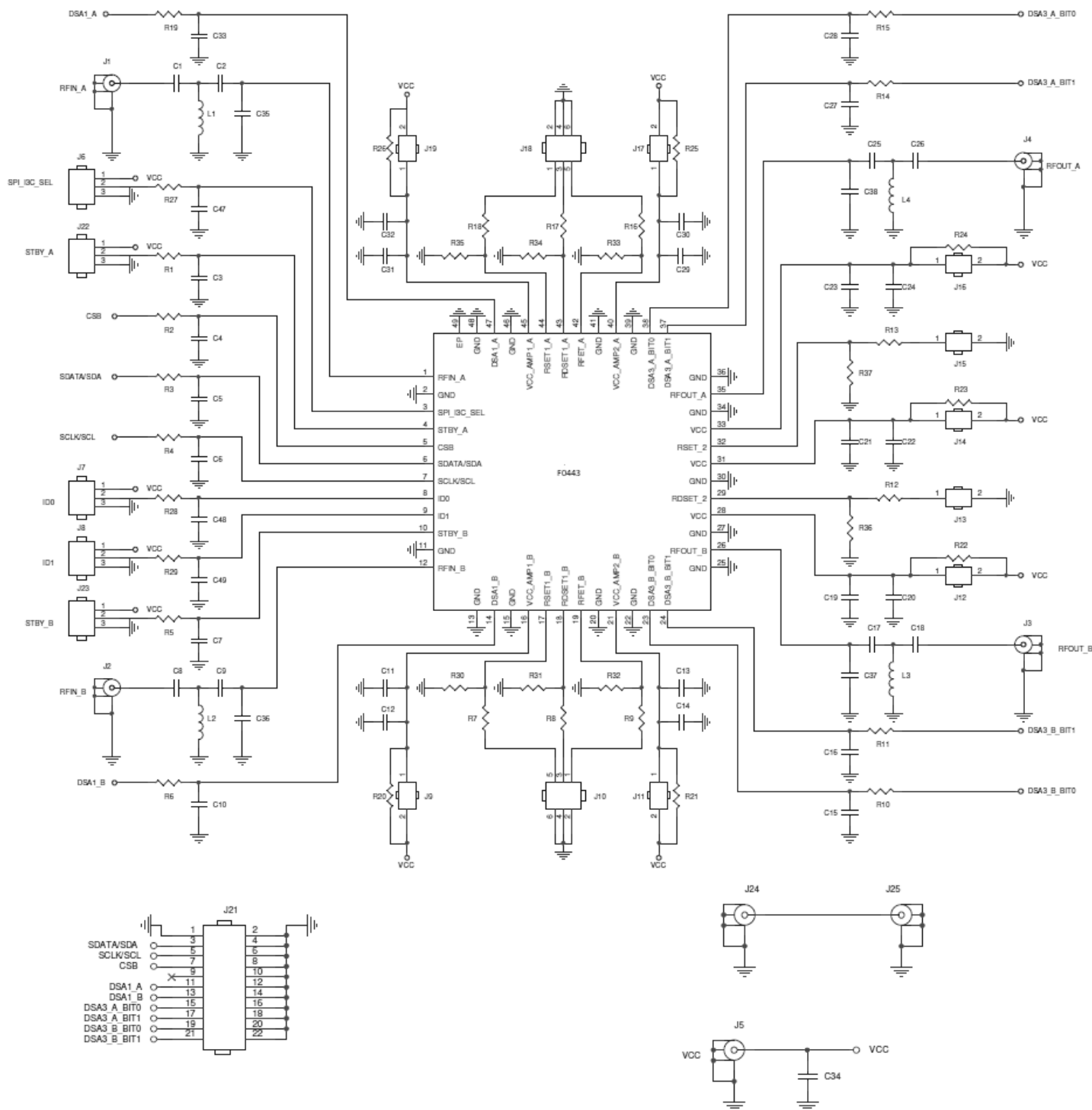
Figure 120. Electrical Schematic
