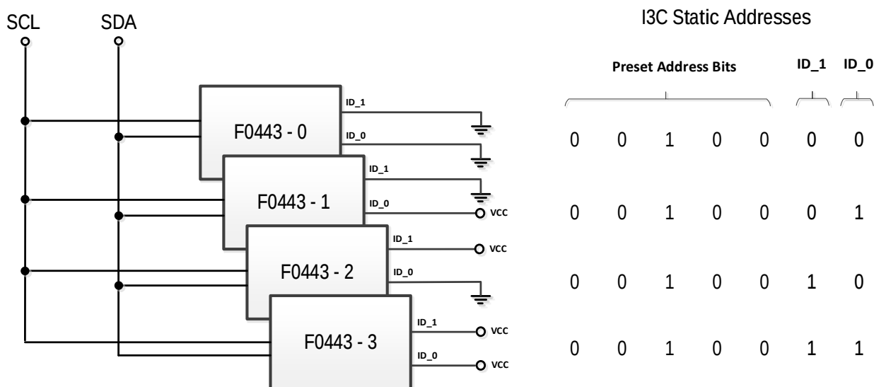
Figure 110. I3C Static Addressing Scheme
