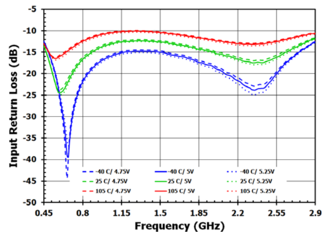
Figure 62. S11, DSA3 = 18dB, Bypass OFF
