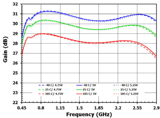
Figure 5. Gain, DSA0 = 6dB, Bypass OFF
