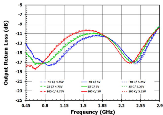
Figure 66. S22, DSA0 = 6dB, Bypass OFF
