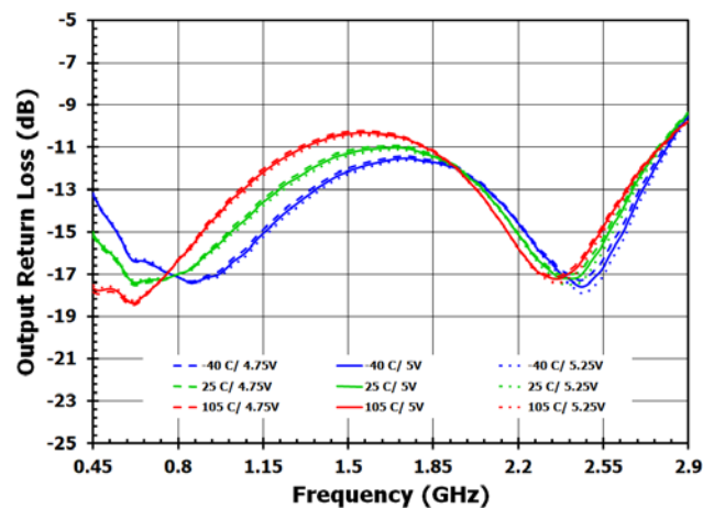
Figure 68. S22, DSA1 = 6dB, Bypass OFF
