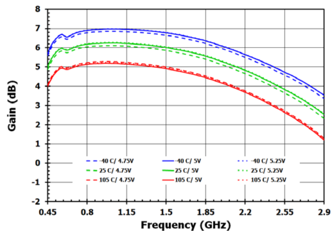
Figure 12. Gain, DSA2 = 10dB, Bypass ON
