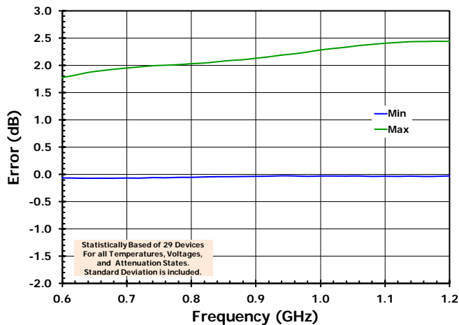
Figure 11. Worse Case Attenuator Absolute Accuracy vs. Freq [All parameters]
