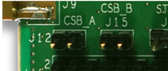
Figure 80. Jumpers for Serial Programming Connections
