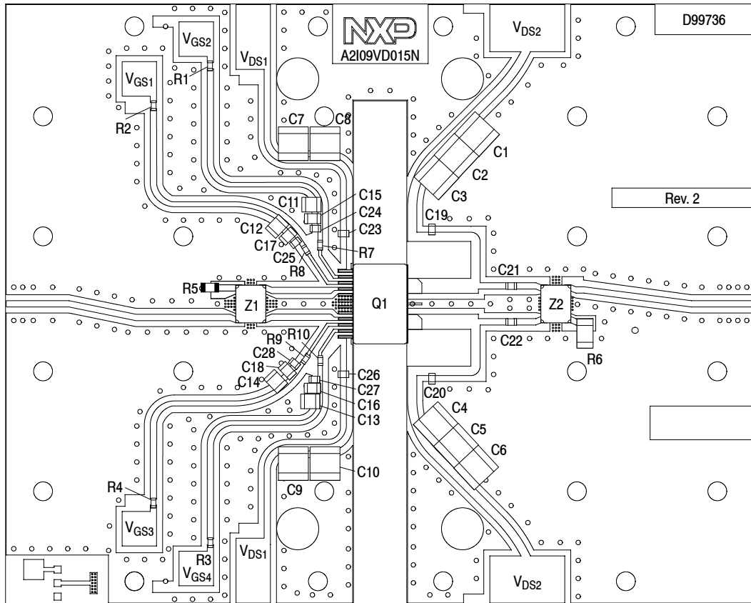
Figure 4. A2109VD015NR1 Characterization Test Circuit Component Layout — 920–960 MHz
