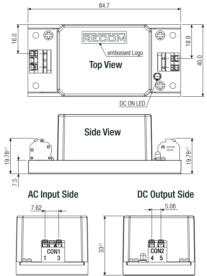
Panel Mount "/PMA" SINGLE Output (mm)
