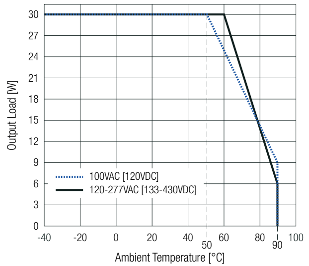
RACM30-xxS(D)K/277 (W; /PMP; /PMA) others
