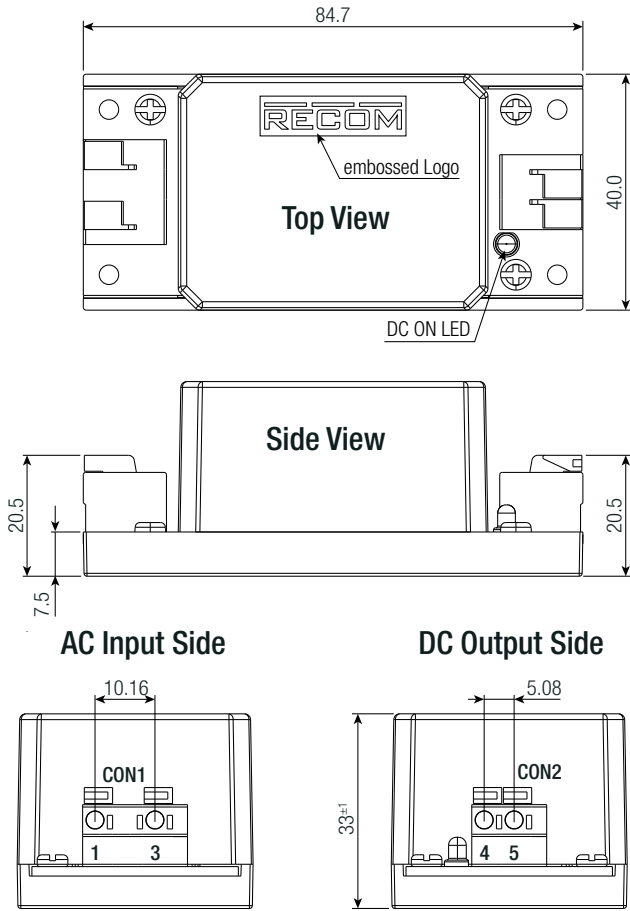
Panel Mount "/PMP" SINGLE Output (mm)
