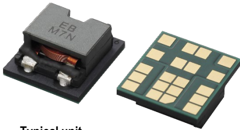
Typical unit
