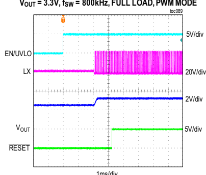
MAXM17633/MAXM17635 STARTUP THROUGH ENABLE (2.5V PREBIAS) V_{OUT} = 3.3V , f_{SW} = 800kHz , FULL LOAD, PWM MODE
