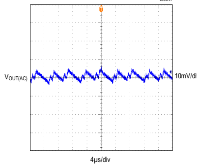
MAXM17634/MAXM17635 STEADY-STATE OUTPUT-VOLTAGE RIPPLE V_{OUT} = 5V , f_{SW} = 1MHz , 20mA LOAD, DCM MODE
