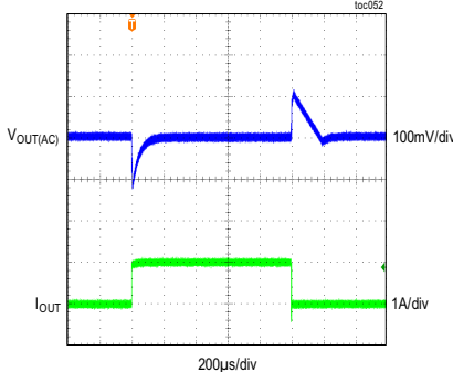
MAXM17635 LOAD-TRANSIENT RESPONSE V_{OUT} = 2.5V , f_{SW} = 700kHz , DCM MODE, LOAD CURRENT STEPPED FROM 20mA TO 1A
