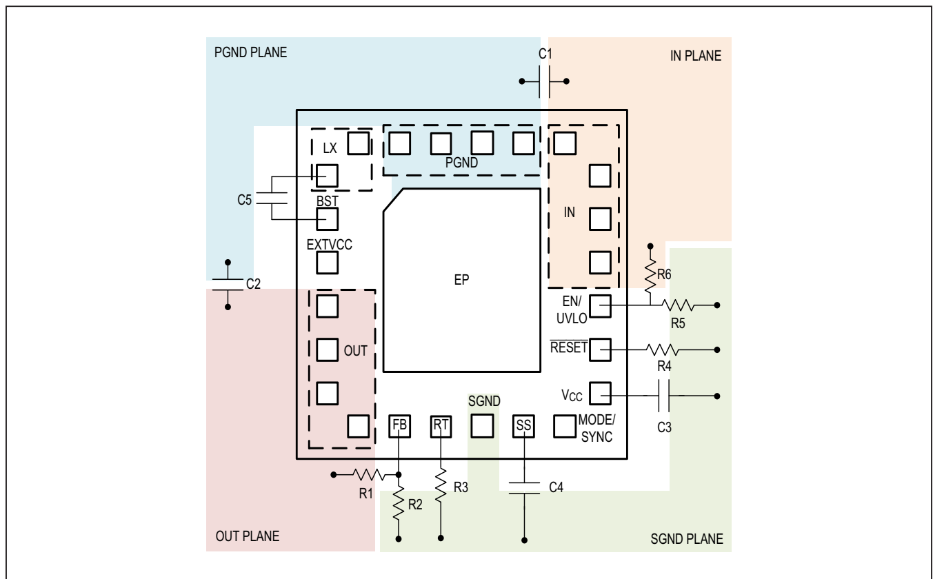
Figure 3. Layout Guidelines
