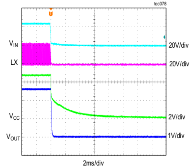
MAXM17635 SHUTDOWN THROUGH IN V_{OUT} = 2.5V , f_{SW} = 700kHz , FULL LOAD, PWM MODE
