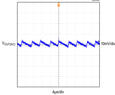
MAXM17633/MAXM17635 STEADY-STATE OUTPUT-VOLTAGE RIPPLE V_{OUT} = 3.3V , f_{SW} = 800kHz , 20mA LOAD, DCM MODE
