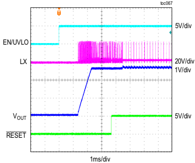
MAXM17635 STARTUP THROUGH ENABLE V_{OUT} = 2.5V , f_{SW} = 700kHz , 20mA LOAD, PFM MODE
