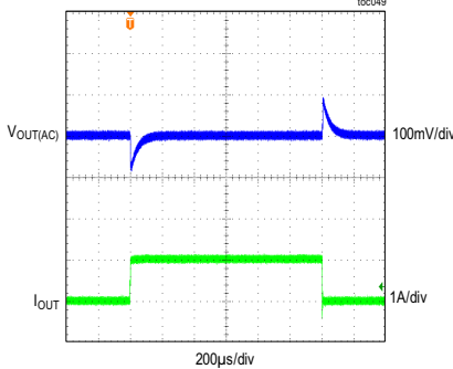
MAXM17635 LOAD-TRANSIENT RESPONSE V_{OUT} = 2.5V , f_{SW} = 700kHz , PWM MODE, LOAD CURRENT STEPPED FROM 0A TO 1A
