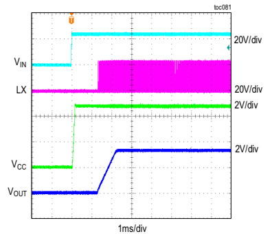
MAXM17633/MAXM17635 STARTUP THROUGH IN V_{OUT} = 3.3V , f_{SW} = 800kHz , FULL LOAD, PWM MODE
