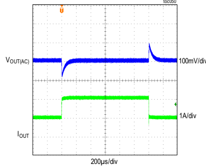
MAXM17635 LOAD-TRANSIENT RESPONSE V_{OUT} = 2.5V , f_{SW} = 700kHz , PWM MODE, LOAD CURRENT STEPPED FROM 1A TO 2A
