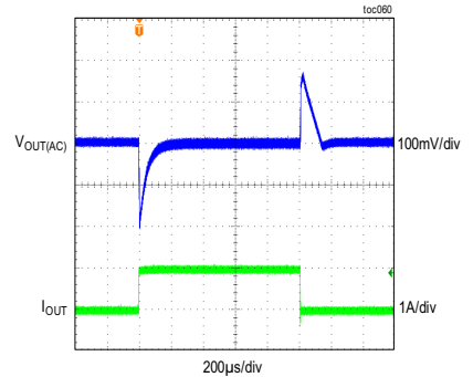
MAXM17634/MAXM17635 LOAD-TRANSIENT RESPONSE V_{OUT} = 5V , f_{SW} = 1MHz , DCM MODE, LOAD CURRENT STEPPED FROM 20mA TO 1A
