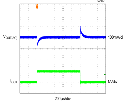
MAXM17633/MAXM17635 LOAD-TRANSIENT RESPONSE V_{OUT} = 3.3V , f_{SW} = 800kHz , PWM MODE, LOAD CURRENT STEPPED FROM 0A TO 1A
