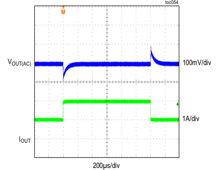
MAXM17633/MAXM17635 LOAD-TRANSIENT RESPONSE V_{OUT} = 3.3V , f_{SW} = 800kHz , PWM MODE, LOAD CURRENT STEPPED FROM 1A TO 2A
