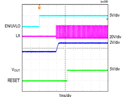
MAXM17634/MAXM17635 STARTUP THROUGH ENABLE (3.3V PREBIAS) V_{OUT} = 5V , f_{SW} = 1MHz , FULL LOAD, PWM MODE
