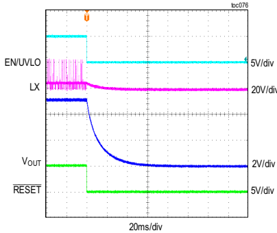
MAXM17634/MAXM17635 SHUTDOWN THROUGH ENABLE V_{OUT} = 5V , f_{SW} = 1MHz , 20mA LOAD, PFM MODE
