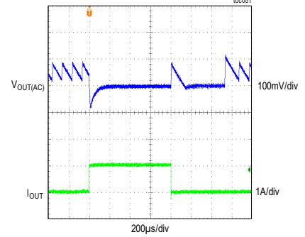
MAXM17635 LOAD-TRANSIENT RESPONSE V_{OUT} = 2.5V , f_{SW} = 700kHz , PFM MODE, LOAD CURRENT STEPPED FROM 20mA TO 1A
