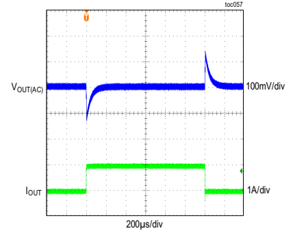
MAXM17634/MAXM17635 LOAD-TRANSIENT RESPONSE V_{OUT} = 5V , f_{SW} = 1MHz , PWM MODE, LOAD CURRENT STEPPED FROM 0A TO 1A
