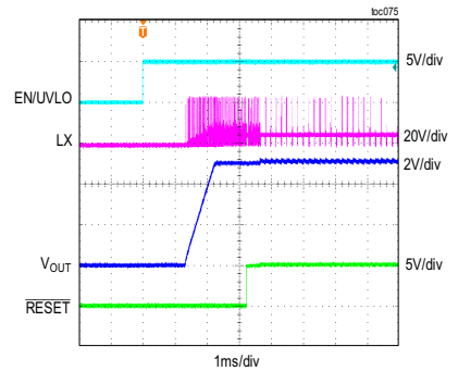
MAXM17634/MAXM17635 STARTUP THROUGH ENABLE V_{OUT} = 5V , f_{SW} = 1MHz , 20mA LOAD, PFM MODE
