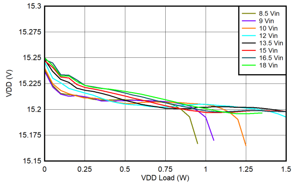
Figure 6-29. UCC14341B-Q1 V_{VDD-VEE} Load Regulation: T_{AMBIENT} = 85^{\circ}C , V_{VDD-VEE} = 15V , V_{COM-VEE} = 4V
