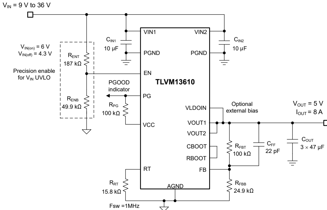
Figure 9-1. Circuit Schematic
