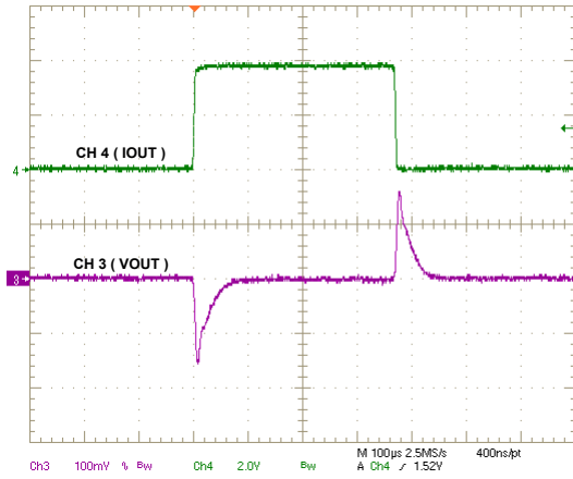
Figure 9-8. Load Transient, 0 A to 4 A, 1 A/µs
