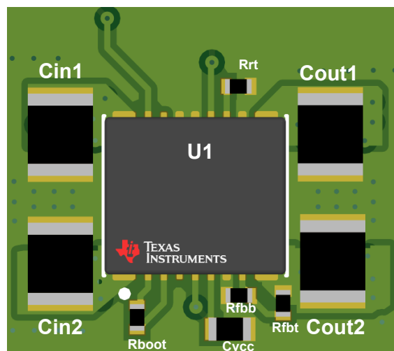
Figure 9-12. Typical Layout
