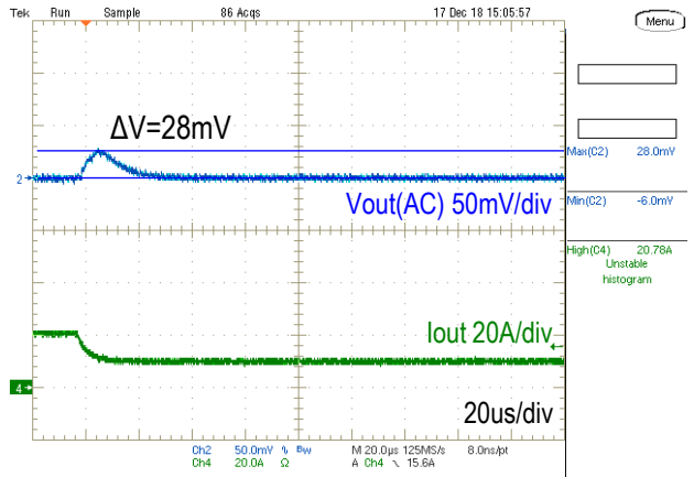
Step Load Transient Response (Vin=12.0V, Vout=0.7V, Cload=660uF, Iout=20 to 10A 1.0A/us) Trace 2=Vout(AC) 50mV/div, Trace 4=Iout 20A/div, 20us/div
