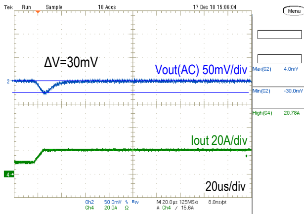
Step Load Transient Response (Vin=12.0V, Vout=0.7V, Cload=660uF, Iout=10A to 20A 1.0A/us) Trace 2=Vout(AC) 50mV/div, Trace 4=Iout 20A/div, 20us/div
