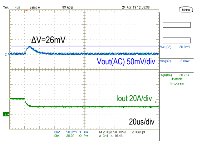
Step Load Transient Response (Vin=5.0V, Vout=0.7V, Cload=660uF, Iout=20 to 10A 1.0A/us) Trace 2=Vout(AC) 50mV/div, Trace 4=Iout 20A/div, 20us/div
