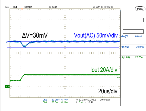
Step Load Transient Response (Vin=5.0V, Vout=0.7V, Cload=660uF, Iout=10A to 20A 1.0A/us) Trace 2=Vout(AC) 50mV/div, Trace 4=Iout 20A/div, 20us/div
