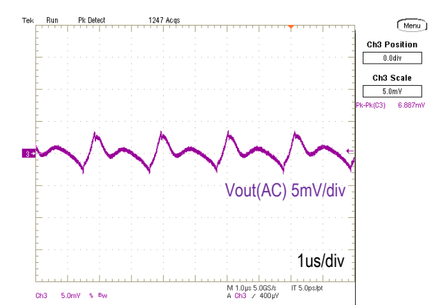
Output Ripple and Noise (Vin=5.0V, Vout=0.7V, Iout=20A, Cload=660uF, Scope BW=20MHz, 5mV/div, 1us/div)
