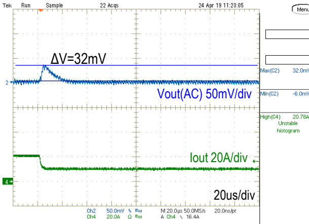
Step Load Transient Response (Vin=5.0V, Vout=1.8V, Cload=660uF, Iout=20 to 10A, 1.0A/us) Trace 2=Vout(AC), 50mV/div, Trace 4=Iout, 20A/div, 20us/div
