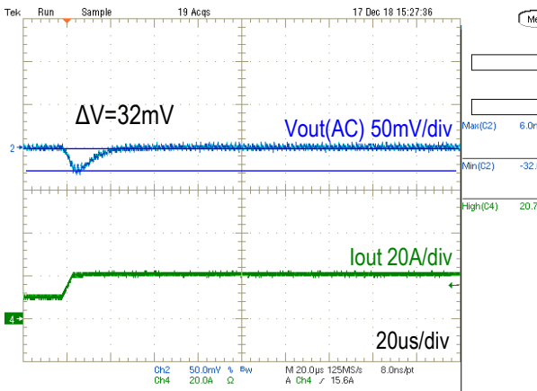
Step Load Transient Response (Vin=12.0V, Vout=1.0V, Cload=660uF, Iout=10A to 20A, 1.0A/us) Trace 2=Vout(AC), 50mV/div, Trace 4=Iout, 20A/div, 20us/div
