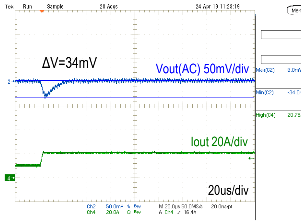
Step Load Transient Response (Vin=5.0V, Vout=1.8V, Cload=660uF, Iout=10A to 20A, 1.0A/us) Trace 2=Vout(AC), 50mV/div, Trace 4=Iout, 20A/div, 20us/div
