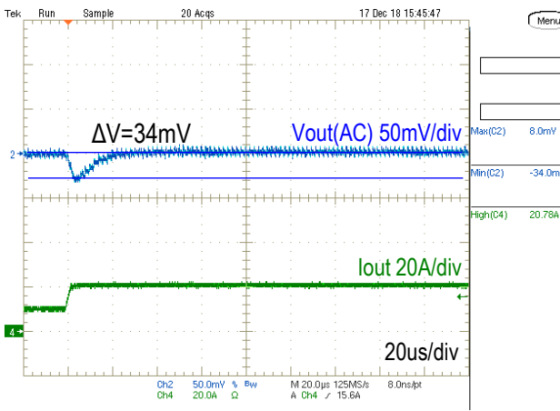
Step Load Transient Response (Vin=12.0V, Vout=1.8V, Cload=660uF, Iout=10A to 20A, 1.0A/us) Trace 2=Vout(AC), 50mV/div, Trace 4=Iout, 20A/div, 20us/div
