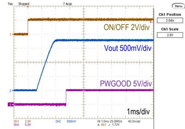
On/Off Enable Delay (Vin=5.0V, Vout=1.8V, Iout=20A, Cload=660uF) Trace1=ON/OFF 2V/div, Trace2=Vout 500mV/div, Trace3=PWGOOD 5V/div, 1ms/div
