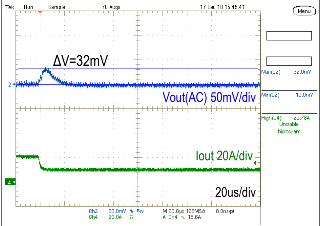
Step Load Transient Response (Vin=12.0V, Vout=1.8V, Cload=660uF, Iout=20 to 10A, 1.0A/us) Trace 2=Vout(AC), 50mV/div, Trace 4=Iout, 20A/div, 20us/div
