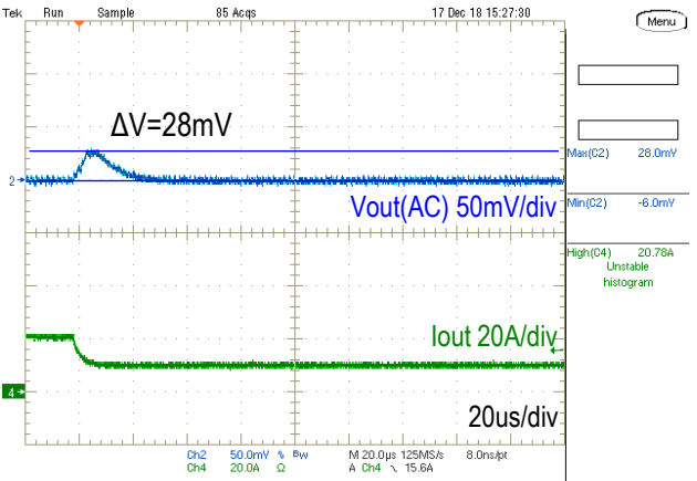
Step Load Transient Response (Vin=12.0V, Vout=1.0V, Cload=660uF, Iout=20 to 10A, 1.0A/us) Trace 2=Vout(AC), 50mV/div, Trace 4=Iout, 20A/div, 20us/div
