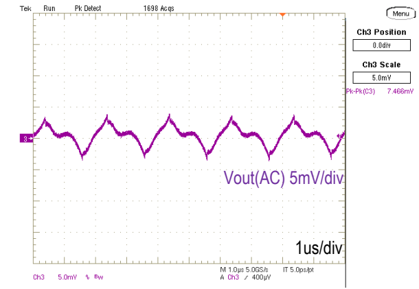
Output Ripple and Noise (Vin=5.0V, Vout=1.8V, Iout=20A, Cload=660uF, Scope BW=20MHz, 5mV/div, 1us/div)
