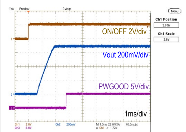
On/Off Enable Delay (Vin=5.0V, Vout=0.7V, Iout=20A, Cload=660uF) Trace1=ON/OFF 2V/div, Trace2=Vout 200mV/div, Trace3=PWGOOD 5V/div, 1ms/div
