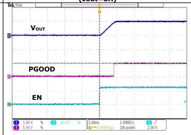
FIG.9 Turn-on (Iout=3A)
