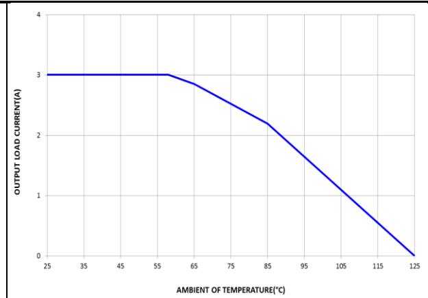
FIG.5 De-rating Curve
