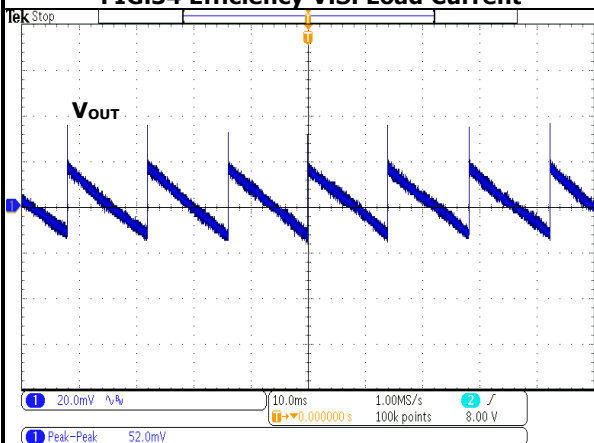
FIG.36 Output Ripple (12Vin, Iout=0A)
