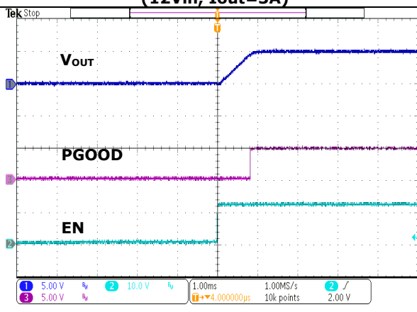
FIG.39 Turn-on (12Vin, Iout=3A)
