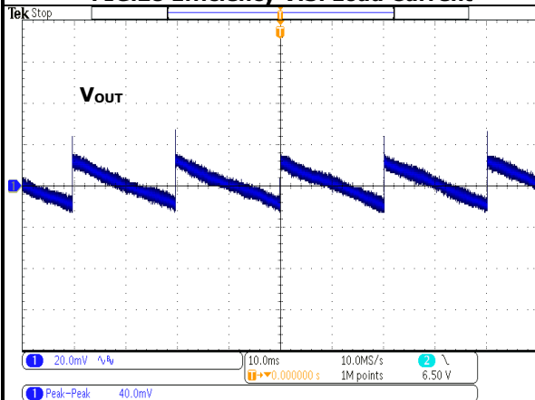
FIG.30 Output Ripple (12Vin, Iout=0A)
