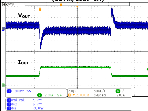
FIG.32 Transient Response (12Vin, 50% to 100% Load Step)
