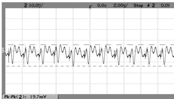
Step Load Transient Response ( V_{in}=12V , V_{out}=1V , C_{load}=0 , I_{out}=3A to 1.5A )
