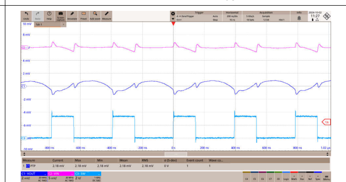
Figure 9-17. PSM Operation I_{OUT} = 0.1A
