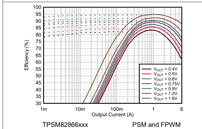
Figure 9-6. Efficiency V_{IN} = 2.8V and T_A = 25^\circ C
