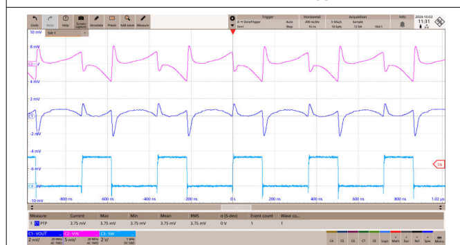
Figure 9-16. FPWM Operation I_{OUT} = 3A
