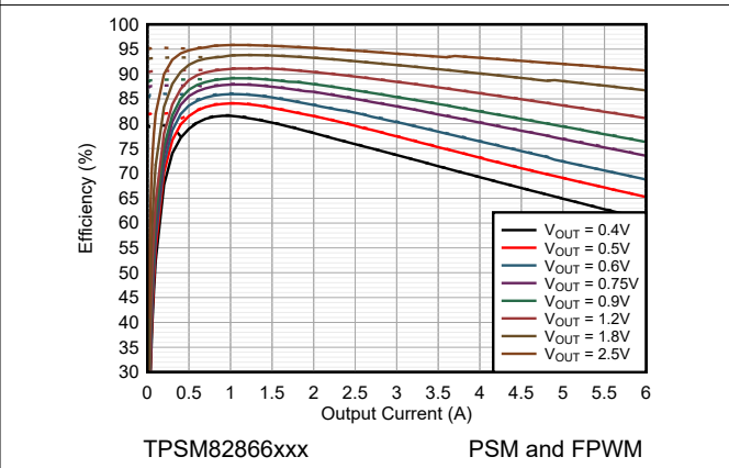
Figure 9-5. Efficiency V_{IN} = 3.3V and T_A = 85^\circ C
