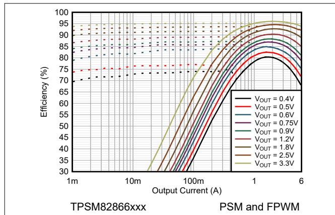
Figure 9-2. Efficiency V_{IN} = 5.0V and T_A = 25^\circ C
