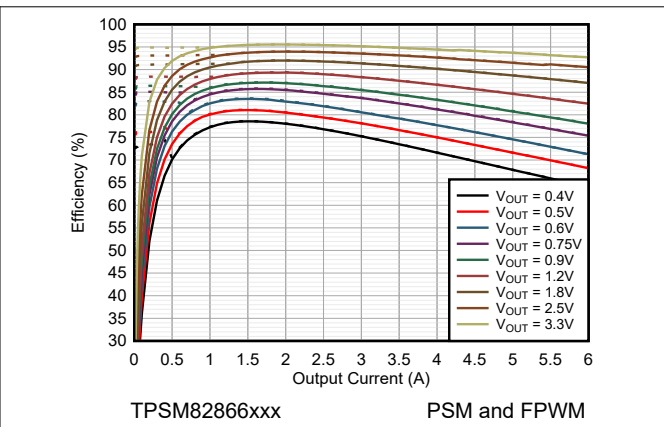
Figure 9-3. Efficiency V_{IN} = 5.0V and T_A = 85^\circ C
