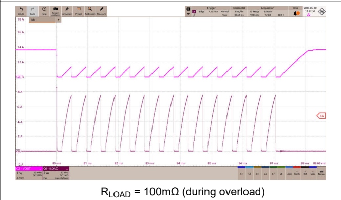
Figure 9-25. HICcup Short-Circuit Protection
