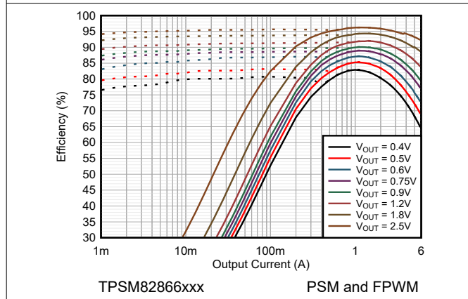
Figure 9-4. Efficiency V_{IN} = 3.3V and T_A = 25^\circ C
