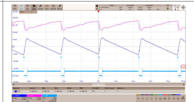
Figure 9-15. Switching Frequency V_{IN} = 3.3V
