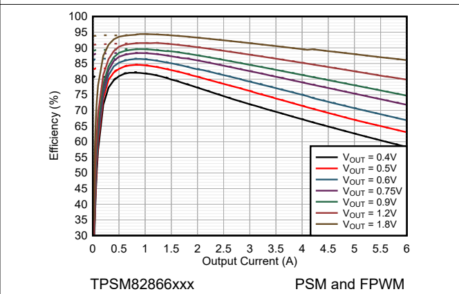
Figure 9-7. Efficiency V_{IN} = 2.8V and T_A = 85^\circ C
