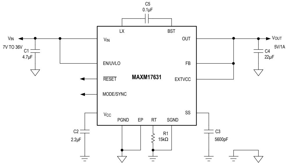
fsw: 1250kHz C1: MURATA 4.7µF/X7R/50V/1206 (GRM31CR71H475KA12) C4: MURATA 22µF/X7R/25V/1210 (GRM32ER71E226KE15)
