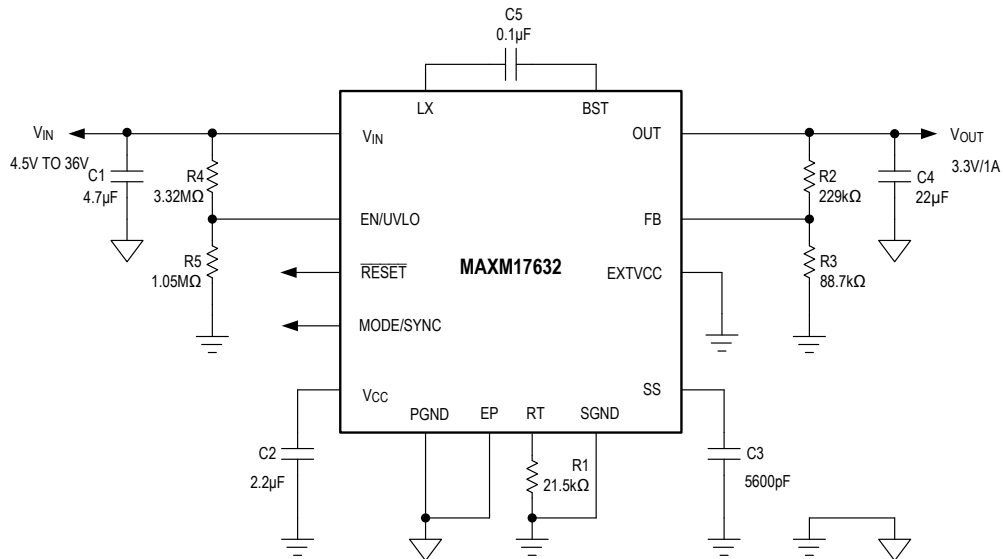
fsw: 900kHz C1: MURATA 4.7µF/X7R/50V/1206 (GRM31CR71H475KA12) C4: MURATA 22µF/X7R/25V/1210 (GRM32ER71E226KE15)
