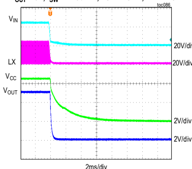
MAXM17631/MAXM17632 SHUTDOWN THROUGH V_{IN} V_{OUT} = 5V , f_{SW} = 1250kHz , FULL LOAD, PWM MODE
