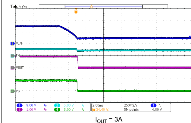
Figure 7-14. VIN Shutdown
