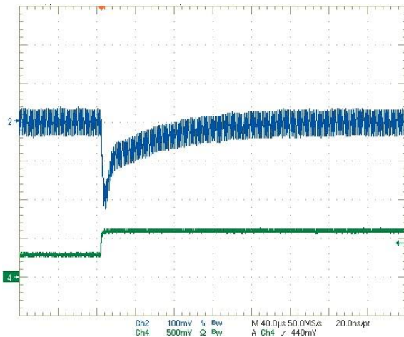
Step Load Transient Response (Vin = 12V, Vout = 5.0V, Cload = 0, Iout = 1.5 to 3A) Trace 2 = Vout, 100 mV/div. Trace 4 = Iout, 2.5A/div.
