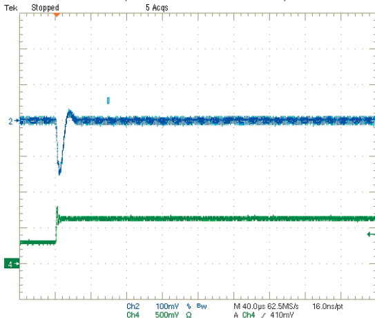
Step Load Transient Response (Vin = 5V, Vout = 1.5V, Clload = 0, Iout = 1.5 to 3A) Trace 2 = Vout, 100 mV/div. Trace 4 = Iout, 2.5A/div.
