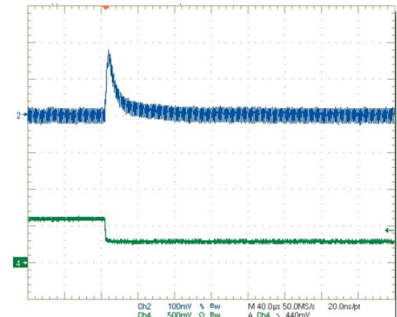
Step Load Transient Response (Vin = 12V, Vout = 2.5V, Cload = 0, Iout = 3 to 1.5A) Trace 2 = Vout, 100 mV/div. Trace 4 = Iout, 2.5A/div.
