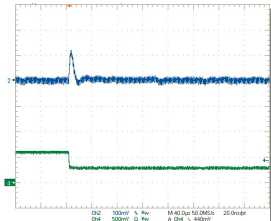
Step Load Transient Response (Vin = 12V, Vout = 1.2V, Clod = 0, Iout = 3 to 1.5A) Trace 2 = Vout, 100 mV/div. Trace 4 = Iout, 2.5A/div.
