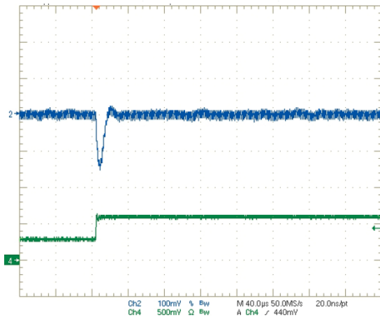
Step Load Transient Response (Vin = 12V, Vout = 1.2V, Clod = 0, Iout = 1.5 to 3A) Trace 2 = Vout, 100 mV/div. Trace 4 = Iout, 2.5A/div.
