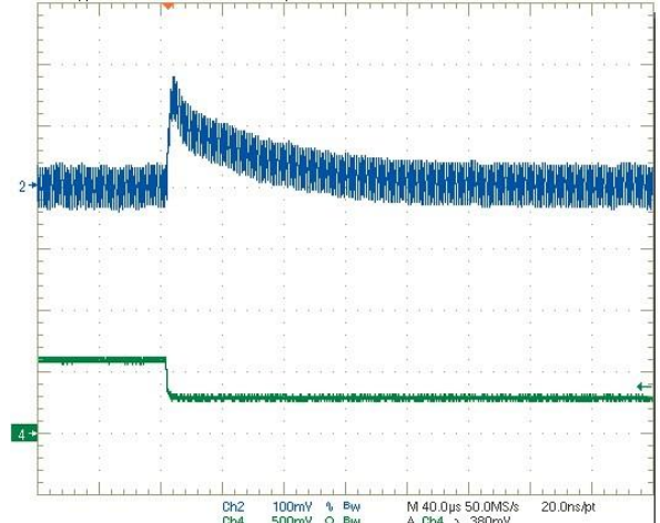
Step Load Transient Response (Vin = 12V, Vout = 5.0V, Cload = 0, Iout = 3 to 1.5A) Trace 2 = Vout, 100 mV/div. Trace 4 = Iout, 2.5A/div.
