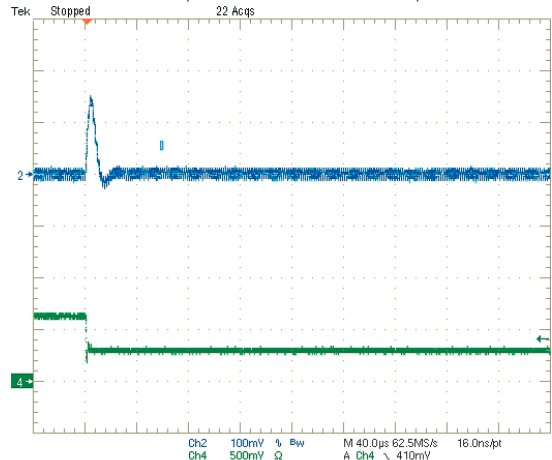
Step Load Transient Response (Vin = 5V, Vout = 1.8V, Clload = 0, Iout = 3 to 1.5A) Trace 2 = Vout, 100 mV/div. Trace 4 = Iout, 2.5A/div.
