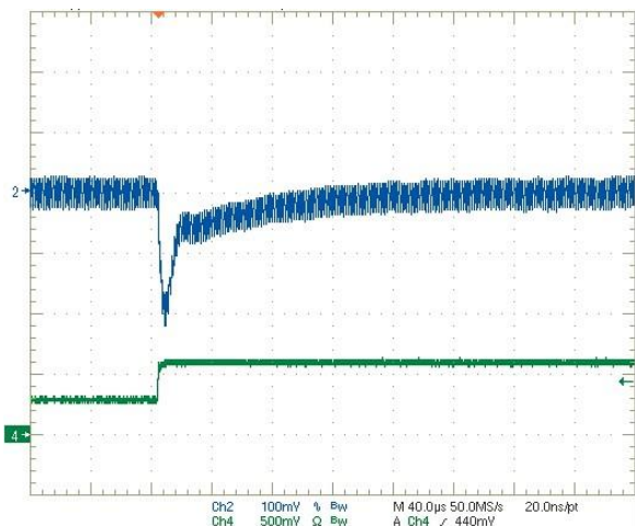
Step Load Transient Response (Vin = 12V, Vout = 3.3V, Cloud = 0, Iout = 1.5 to 3A) Trace 2 = Vout, 100 mV/div. Trace 4 = Iout, 2.5A/div.
