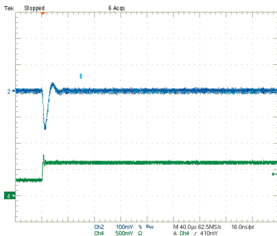
Step Load Transient Response (Vin = 5V, Vout = 1.0V, Cloud = 0, Iout = 1.5 to 3A) Trace 2 = Vout, 100 mV/div. Trace 4 = Iout, 2.5A/div.
