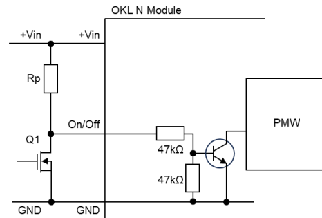
BOM → Rp → 20k BOM → Q1 → Q SMT Nch-MOS 30V
