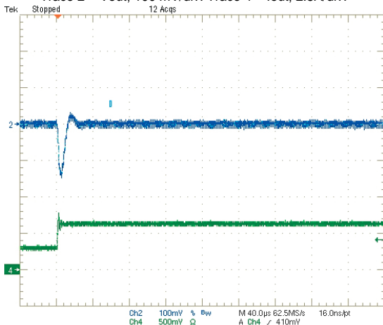
Step Load Transient Response (Vin = 5V, Vout = 1.2V, Clload = 0, Iout = 1.5 to 3A) Trace 2 = Vout, 100 mV/div. Trace 4 = Iout, 2.5A/div.
