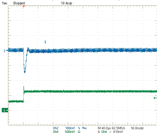
Step Load Transient Response (Vin = 5V, Vout = 3.3V, Clload = 0, Iout = 1.5 to 3A) Trace 2 = Vout, 100 mV/div. Trace 4 = Iout, 2.5A/div.
