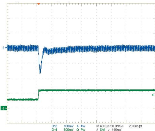
Step Load Transient Response (Vin = 12V, Vout = 2.5V, Cload = 0, Iout = 1.5 to 3A) Trace 2 = Vout, 100 mV/div. Trace 4 = Iout, 2.5A/div.
