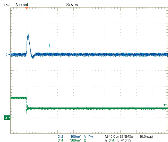
Step Load Transient Response (Vin = 5V, Vout = 1.0V, Cloud = 0, Iout = 3 to 1.5A) Trace 2 = Vout, 100 mV/div. Trace 4 = Iout, 2.5A/div.
