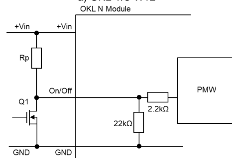
BOM → Rp → 8.2k BOM → Q1 → Q SMT Nch-MOS 30V
