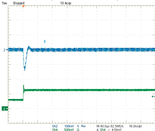
Step Load Transient Response (Vin = 5V, Vout = 1.8V, Clload = 0, Iout = 1.5 to 3A) Trace 2 = Vout, 100 mV/div. Trace 4 = Iout, 2.5A/div.
