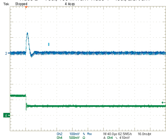
Step Load Transient Response (Vin = 5V, Vout = 1.2V, Clload = 0, Iout = 3 to 1.5A) Trace 2 = Vout, 100 mV/div. Trace 4 = Iout, 2.5A/div.
