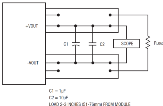
Figure 5. Measuring Output Ripple and Noise (PARD)
