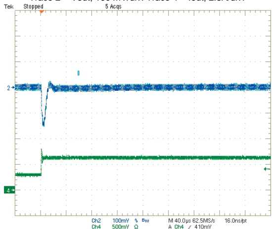
Step Load Transient Response (Vin = 5V, Vout = 2.5V, Clload = 0, Iout = 1.5 to 3A) Trace 2 = Vout, 100 mV/div. Trace 4 = Iout, 2.5A/div.
