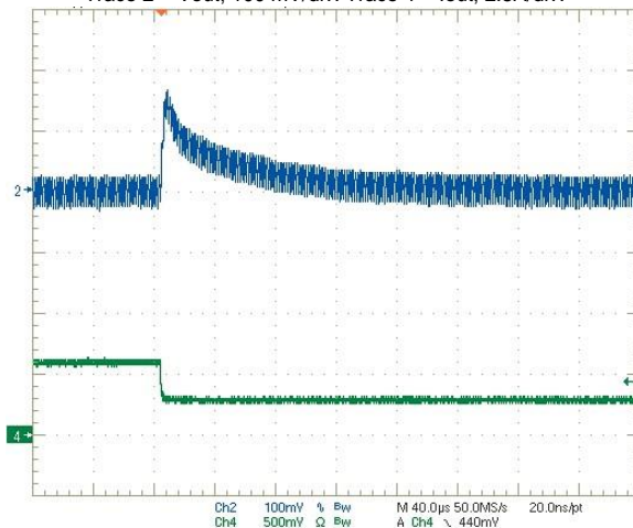
Step Load Transient Response (Vin = 12V, Vout = 3.3V, Cloud = 0, Iout = 3 to 1.5A) Trace 2 = Vout, 100 mV/div. Trace 4 = Iout, 2.5A/div.
