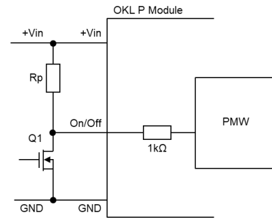
BOM → Rp → 20k BOM → Q1 → Q SMT Nch-MOS 30V
