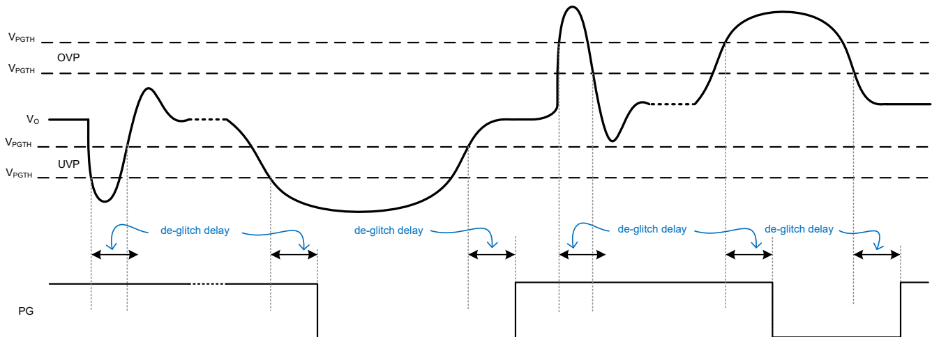
Figure 7-7. Power-Good Behavior
