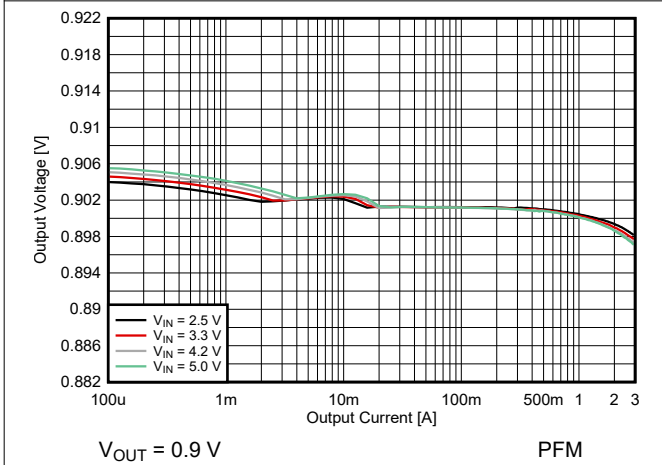
Figure 8-16. Output Voltage versus Output Current
