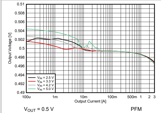
Figure 8-14. Output Voltage versus Output Current
