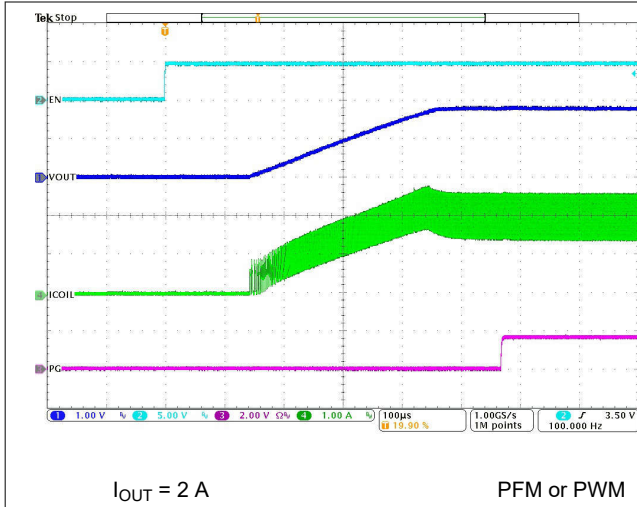
Figure 8-44. Start-Up With Load
