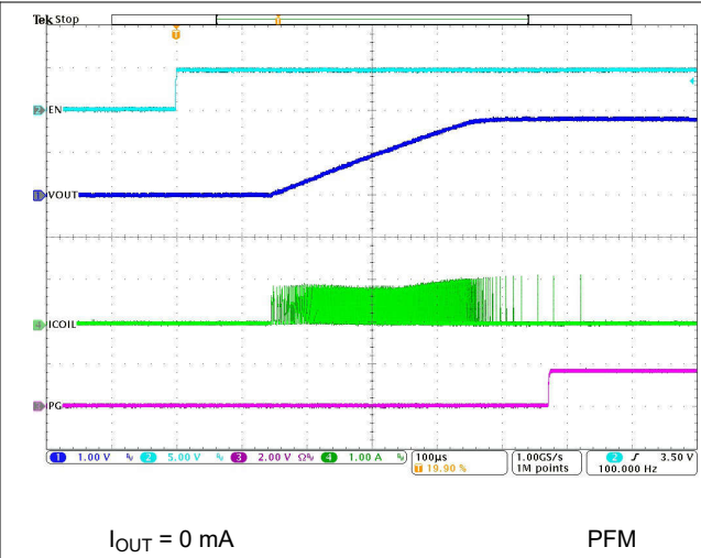
Figure 8-45. Start-Up With No Load
