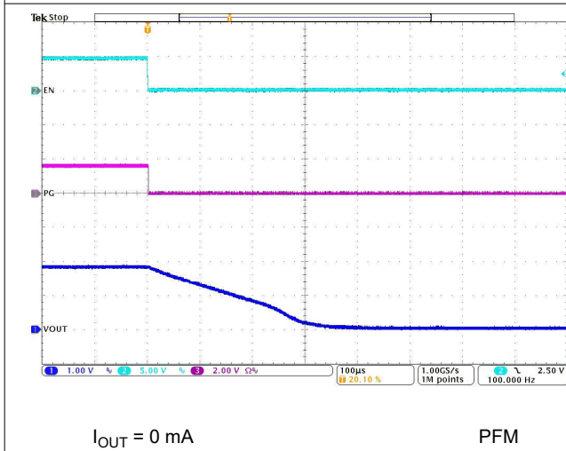
Figure 8-46. Disable, Active Output Discharge at No Load
