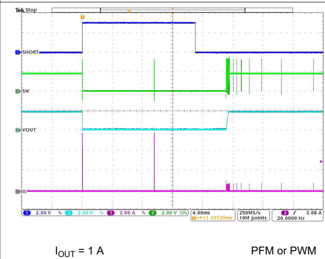
Figure 8-47. HICCUP Short-Circuit Protection
