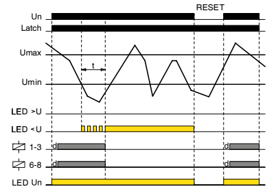
UL UNDER + Latch
