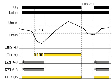
WL WINDOW + Latch
