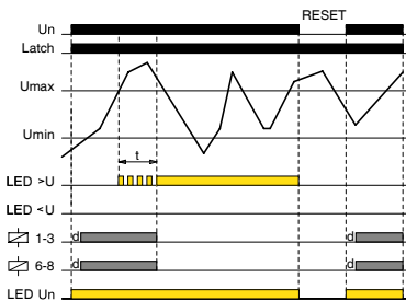
OL OVER + Latch
