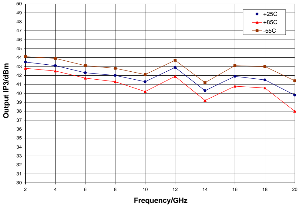
Output IP3, V_{dd} = 28\text{ V} , V_{gg1} = -2.8\text{ V} , V_{gg2} = 10\text{ V} , I_{dd} = 700\text{ mA} , T_A = 25\text{ °C}
