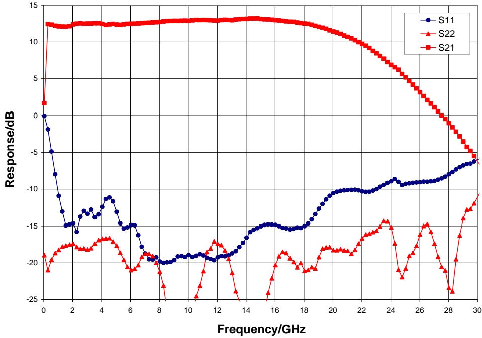
Broadband Performance, V_{dd} = 28\text{ V} , V_{gg1} = -2.8\text{ V} , V_{gg2} = 10\text{ V} , I_{dd} = 700\text{ mA} , T_A = 25\text{ }^\circ\text{C}
