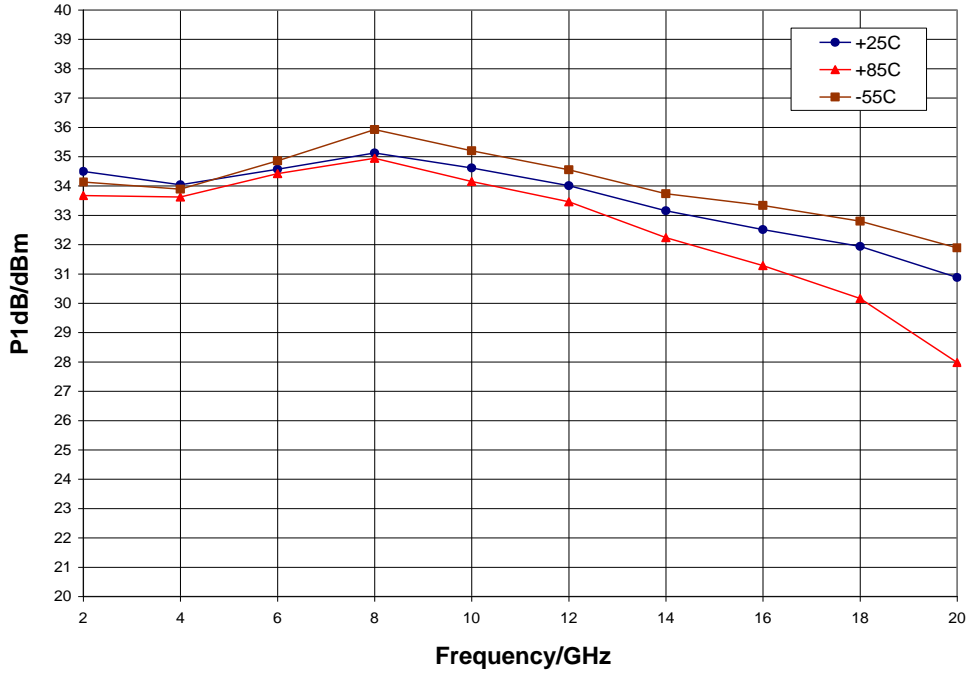
P1dB vs. Temperature, V_{dd} = 28\text{ V} , V_{gg1} = -2.8\text{ V} , V_{gg2} = 10\text{ V}
