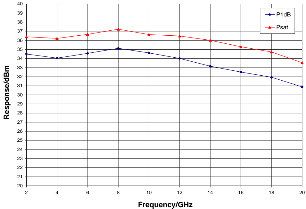
Output Power, V_{dd} = 28\text{ V} , V_{gg1} = -2.8\text{ V} , V_{gg2} = 10\text{ V} , T_A = 25\text{ °C}
