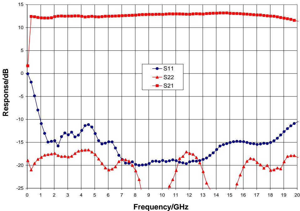
Narrow-band Performance, V_{dd} = 28\text{ V} , V_{gg1} = -2.8\text{ V} , V_{gg2} = 10\text{ V} , I_{dd} = 700\text{ mA} , T_A = 25\text{ }^\circ\text{C}
