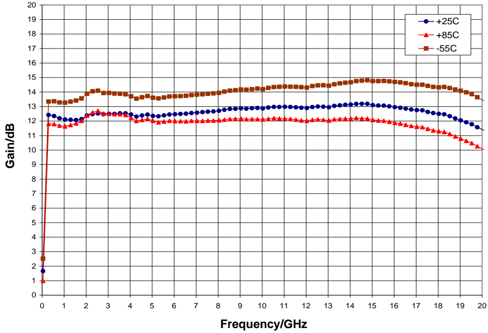
Gain vs. Temperature, V_{dd} = 28\text{ V} , V_{gg1} = -2.8\text{ V} , V_{gg2} = 10\text{ V}
