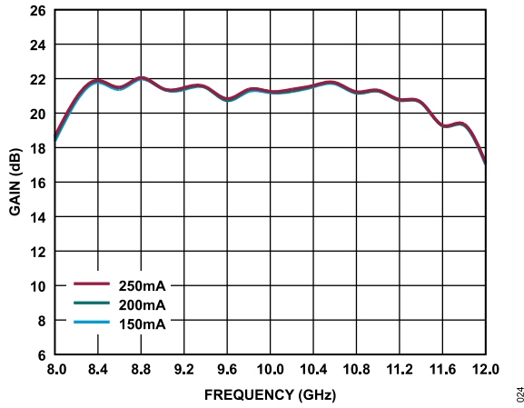
Figure 17. Gain at P_{IN} = 22 \text{ dBm} vs. Frequency for Various I_{DQ} Values at V_{DD} = 28 \text{ V}
