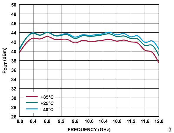
Figure 21. P_{OUT} vs. Frequency for Various Temperatures at P_{IN} = 22 \text{ dBm}
