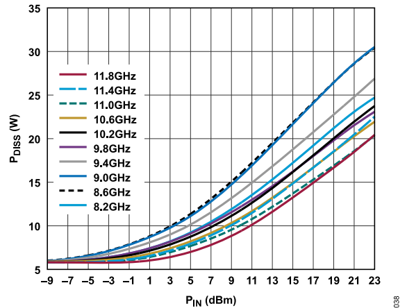
Figure 38. P_{DISS} vs. P_{IN} for Various Frequencies, Pulse Width = 100 \mu s at 20% Duty Cycle
