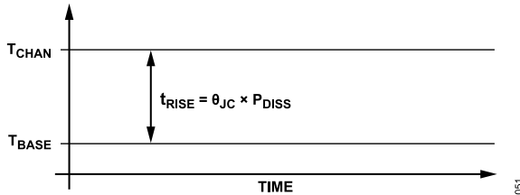
Figure 48. Channel Temperature Rise for Continuous Bias Condition
