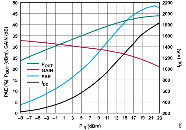
Figure 31. P_{AE} , P_{OUT} , Gain, and Supply Current ( I_{DD} ) vs. P_{IN} at 8.4 GHz
