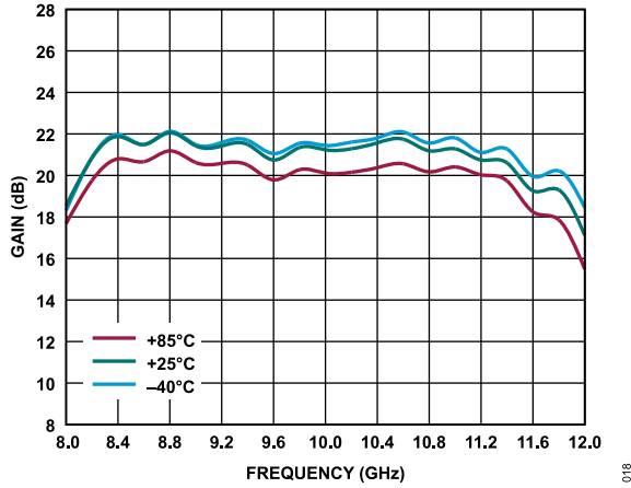
Figure 16. Gain vs. Frequency for Various Temperatures at P_{IN} = 22 \text{ dBm}
