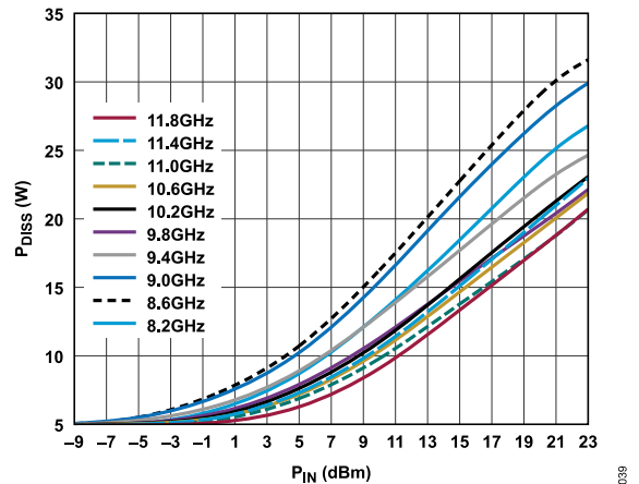
Figure 39. P_{DISS} vs. P_{IN} for Various Frequencies, Pulse Width = 300 \mu s at 10% Duty Cycle
