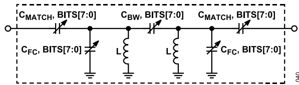
Figure 18. Simplified Filter Architecture Diagram
