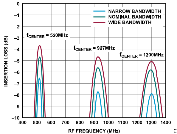
Figure 15. Insertion Loss vs. RF Frequency at Various Bandwidths and Center Frequencies
