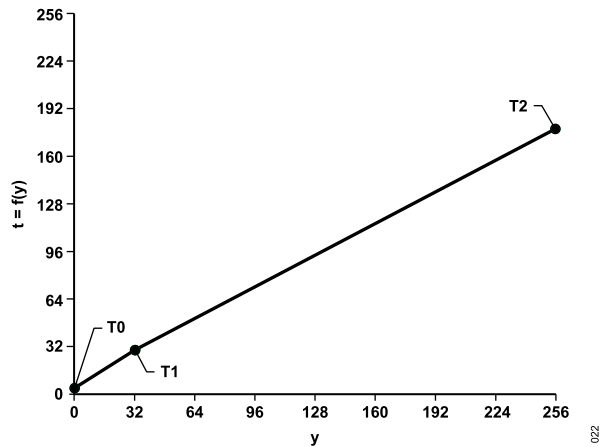
Figure 24. Interpolation Function of t = f(y)
