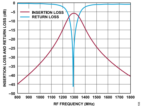
Figure 8. Insertion Loss and Return Loss vs. RF Frequency for Nominal Bandwidth at 1.3 GHz
