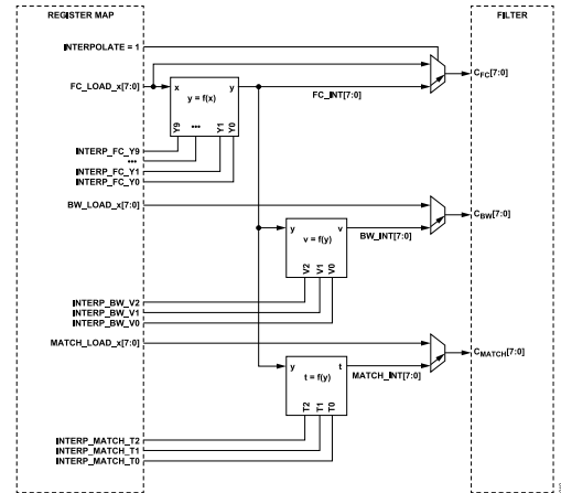
Figure 21. Interpolation Diagram
