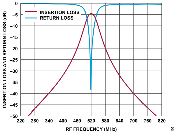
Figure 5. Insertion Loss and Return Loss vs. RF Frequency for Nominal Bandwidth at 520 MHz
