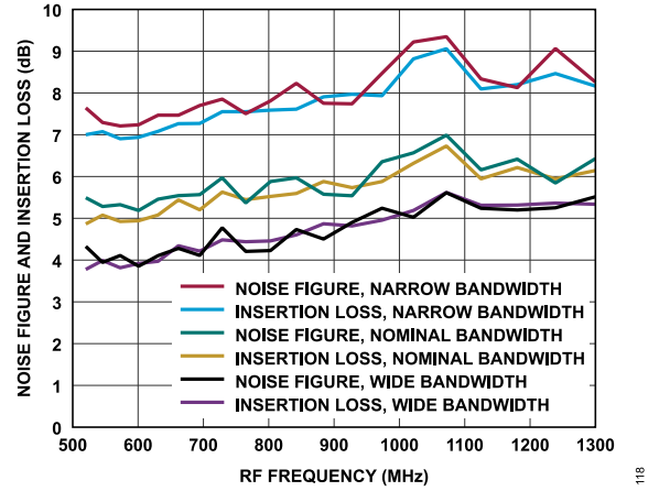
Figure 17. Noise Figure and Insertion Loss vs. RF Frequency for Various Bandwidths
