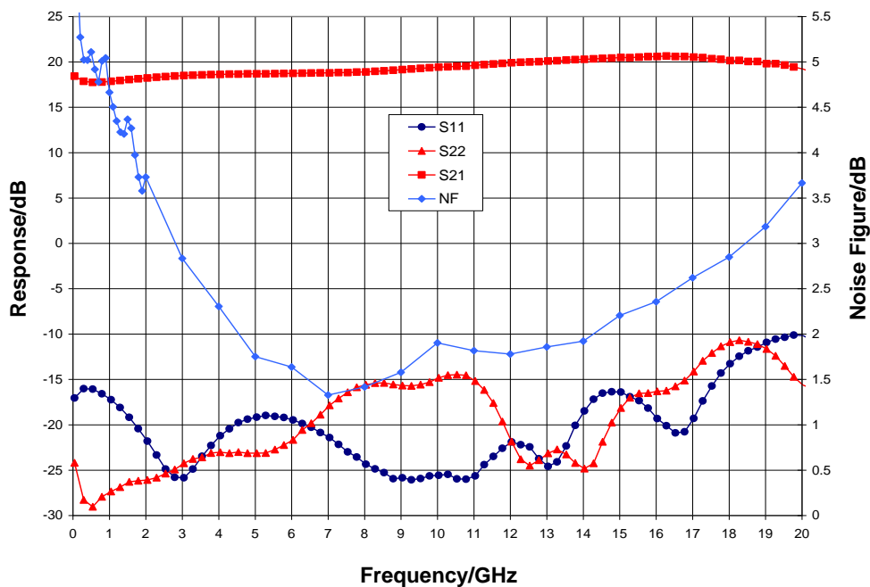
Narrow-band Performance, V_{dd} = 8.0\text{ V} , V_{gg} = -1.0\text{ V} , I_{dd} = 170\text{ mA} , T_A = 25\text{ }^\circ\text{C}
