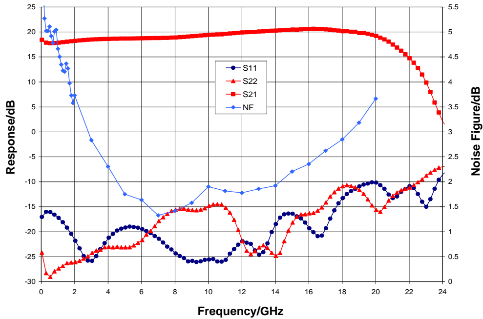
Broadband Performance, V_{dd} = 8.0\text{ V} , V_{gg} = -1.0\text{ V} , I_{dd} = 170\text{ mA} , T_A = 25\text{ }^\circ\text{C}
