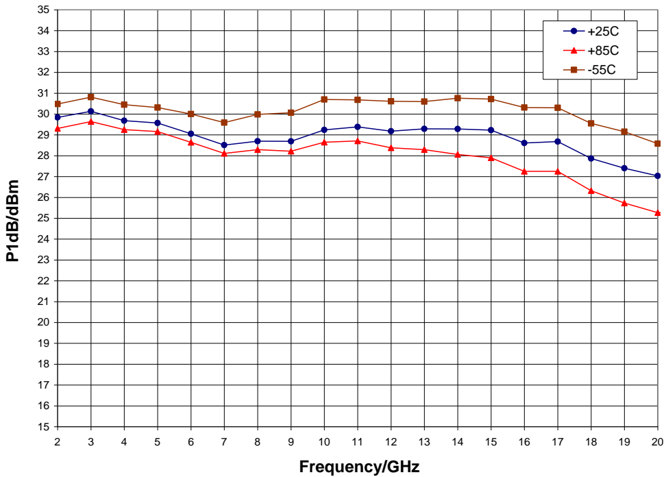
P1dB vs. Temperature, V_{dd} = 10\text{ V} , V_{gg1} = -0.55\text{ V} , V_{gg2} = 5\text{ V}
