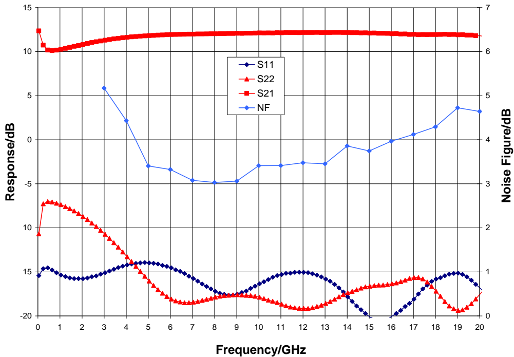
Narrow-band Performance, V_{dd} = 10\text{ V} , V_{gg1} = -0.55\text{ V} , V_{gg2} = 5\text{ V} , I_{dd} = 400\text{ mA} , T = 25\text{ }^\circ\text{C}
