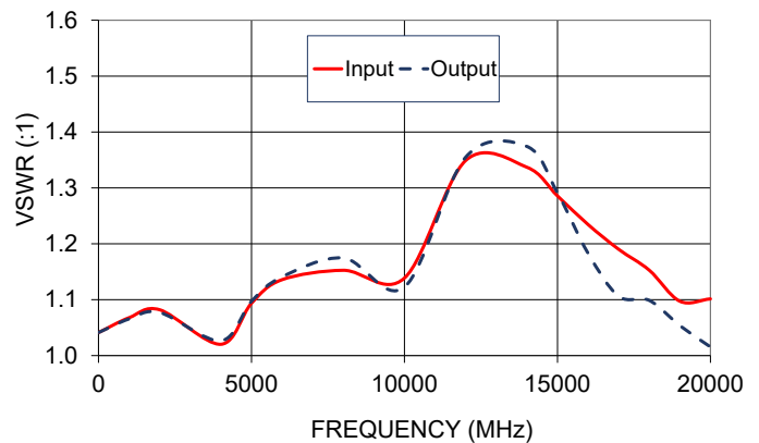
EQY-2-24+ VSWR
