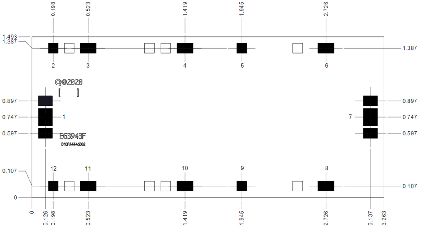
Dimensions: mm; Thickness: 0.05 mm; Die x, y size tolerance: ± 0.050; Ground is backside of die
