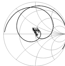
Freq ( 0.01GHz to 4.00GHz )
