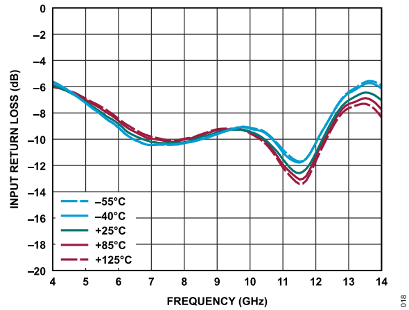
Figure 18. Input Return Loss vs. Frequency for Various Temperatures, 4 GHz to 14 GHz, V_{DD} = 3\text{ V} , I_{DQ} = 60\text{ mA} , and R_{BIAS} = 470\ \Omega
