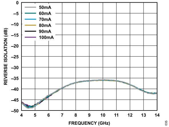
Figure 35. Reverse Isolation vs. Frequency for Various I_{DQ} Values, 4 GHz to 14 GHz, and V_{DD} = 3\text{ V}
