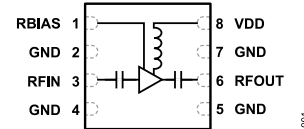
Figure 1. Functional Block Diagram
