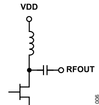
Figure 6. VDD and RFOUT Interface Schematic
