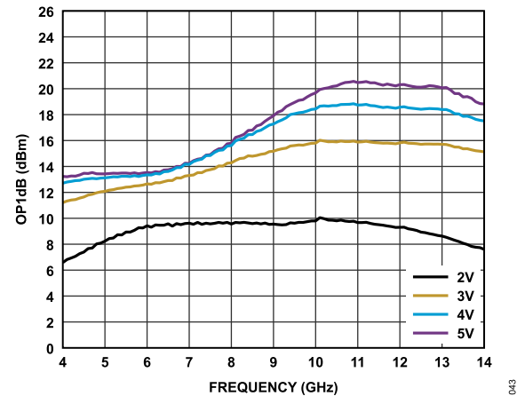
Figure 43. OP1dB vs. Frequency for Various Supply Voltages, 4 GHz to 14 GHz, and I_{DQ} = 60\text{ mA}
