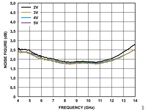
Figure 37. Noise Figure vs. Frequency for Various Supply Voltages, 4 GHz to 14 GHz, and I_{DQ} = 60\text{ mA}
