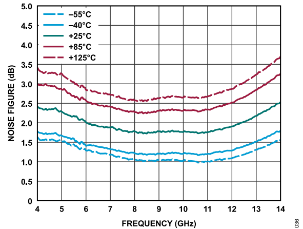
Figure 36. Noise Figure vs. Frequency for Various Temperatures, 4 GHz to 14 GHz, V_{DD} = 3\text{ V} , I_{DQ} = 60\text{ mA} , and R_{BIAS} = 470\ \Omega
