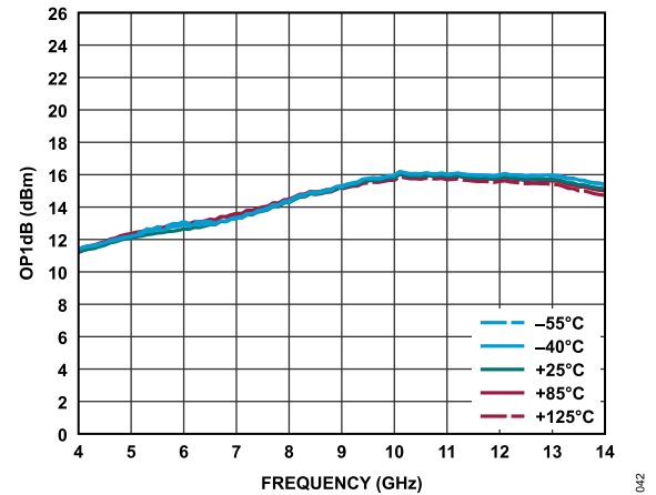
Figure 42. OP1dB vs. Frequency for Various Temperatures, 4 GHz to 14 GHz, V_{DD} = 3\text{ V} , I_{DQ} = 60\text{ mA} , and R_{BIAS} = 470\ \Omega
