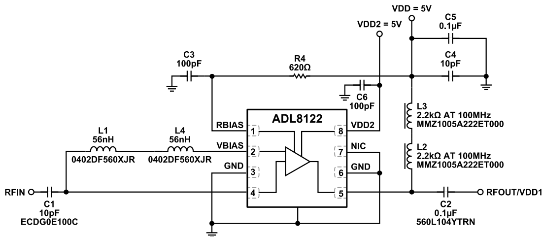
Figure 99. Application Circuit for ADL8122-EVALZ Optimized Overdrive Recovery Time
