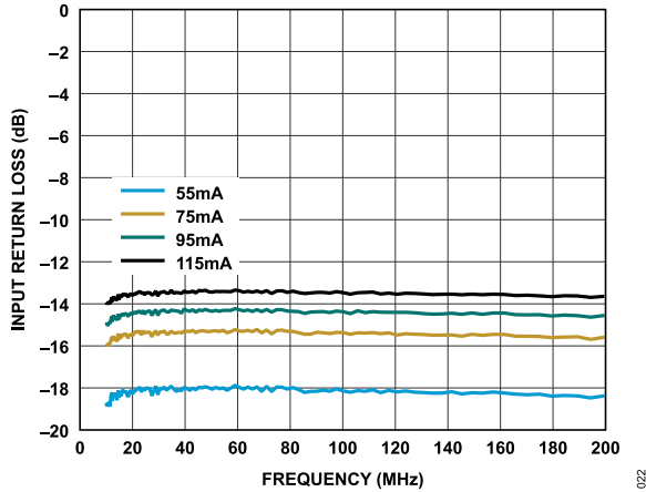
Figure 22. Input Return Loss vs. Frequency for Various I_{DQ} Values, 10 MHz to 200 MHz, V_{DD} = 5\text{ V}
