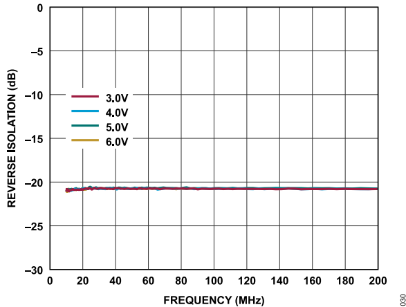
Figure 30. Reverse Isolation vs. Frequency for Various Supply Voltages, 10 MHz to 200 MHz, I_{DQ} = 95\text{ mA}
