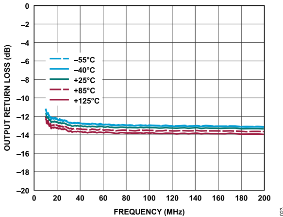
Figure 23. Output Return Loss vs. Frequency for Various Temperatures, 10 MHz to 200 MHz, V_{DD} = 5\text{ V} , I_{DQ} = 95\text{ mA} , R_{BIAS} = 620\ \Omega
