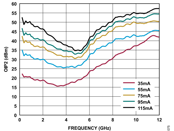
Figure 75. OIP2 vs. Frequency for Various I_{DQ} Values, 200 MHz to 12 GHz, V_{DD} = 5\text{ V}
