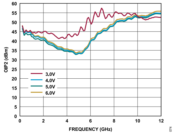
Figure 74. OIP2 vs. Frequency for Various Supply Voltages, 200 MHz to 12 GHz, I_{DQ} = 95\text{ mA}
