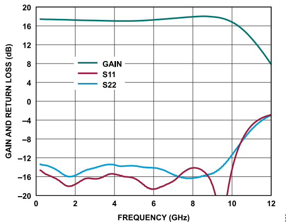
Figure 93. Gain and Return Loss vs. Frequency of 10 MHz to 12 GHz Application Circuit, 200 MHz to 12 GHz, V_{DD} = 5\text{ V} , I_{DQ} = 95\text{ mA} , R_{BIAS} = 620\ \Omega
