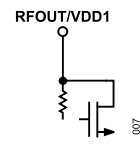
Figure 8. RFOUT/VDD1 Interface Schematic
