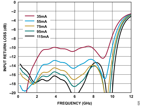
Figure 25. Input Return Loss vs. Frequency for Various I_{DQ} Values, 200 MHz to 12 GHz, V_{DD} = 5\text{ V}
