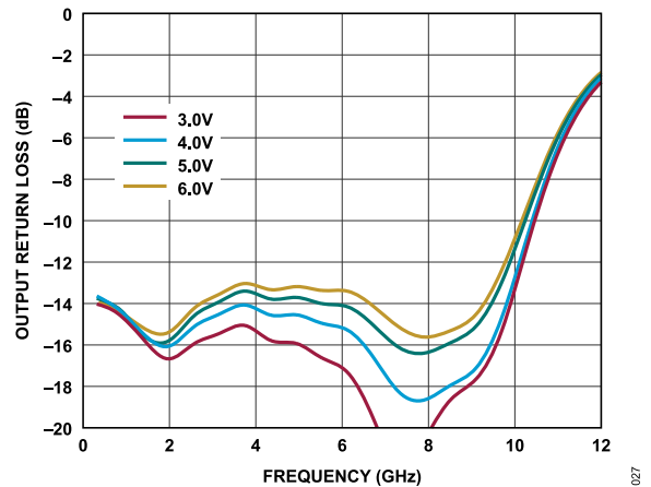
Figure 27. Output Return Loss vs. Frequency for Various Supply Voltages, 200 MHz to 12 GHz, I_{DQ} = 95\text{ mA}
