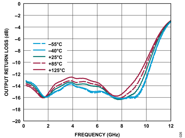
Figure 26. Output Return Loss vs. Frequency for Various Temperatures, 200 MHz to 12 GHz, V_{DD} = 5\text{ V} , I_{DQ} = 95\text{ mA} , R_{BIAS} = 620\ \Omega
