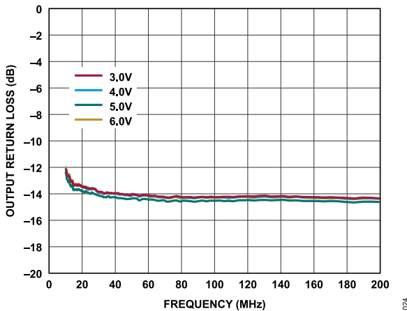
Figure 24. Output Return Loss vs. Frequency for Various Supply Voltages, 10 MHz to 200 MHz, I_{DQ} = 95\text{ mA}
