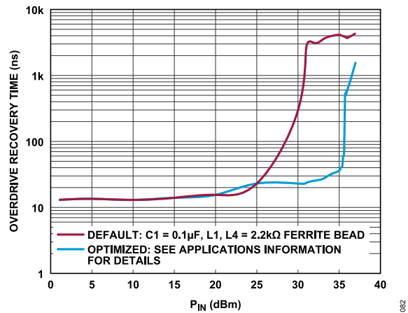
Figure 82. Overdrive Recovery Time vs. P_{IN} at 6 GHz, Recovery Time to Within 90% of Small Signal Gain Value, V_{DD} = 5\text{ V} , R_{BIAS} = 620\ \Omega
