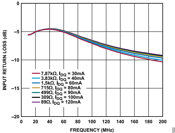
Figure 22. Input Return Loss vs. Frequency for Various R_{BIAS} and I_{DQ} Values, V_{DD} = 5 \text{ V} , 10 MHz to 200 MHz
