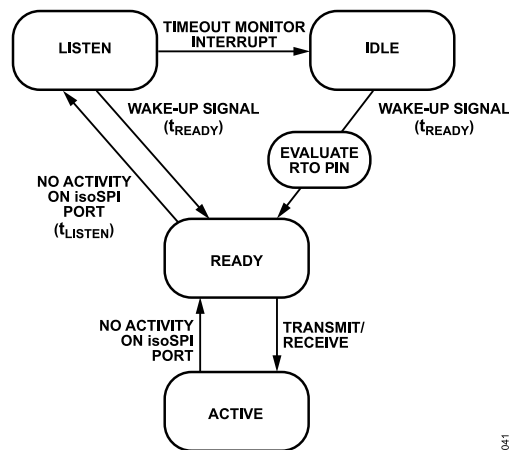
Figure 42. LPCM Expanded State Diagram
