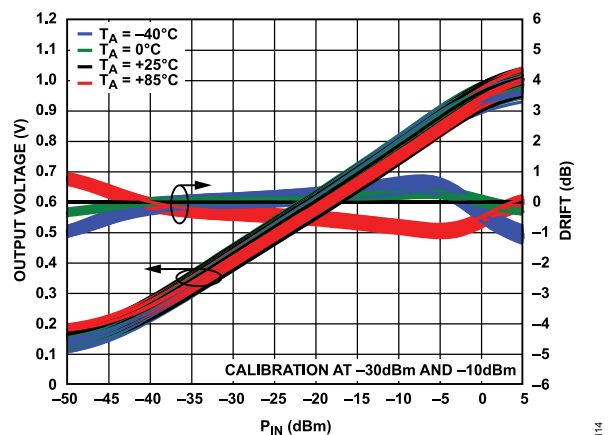
Figure 14. Distribution of Log Conformance Error with Respect to V_{LOG} at 25°C vs. P_{IN} and Temperature at 100 MHz
