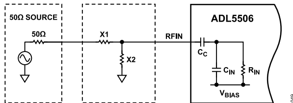
Figure 47. Narrow-Band Reactive Method for Input Coupling
