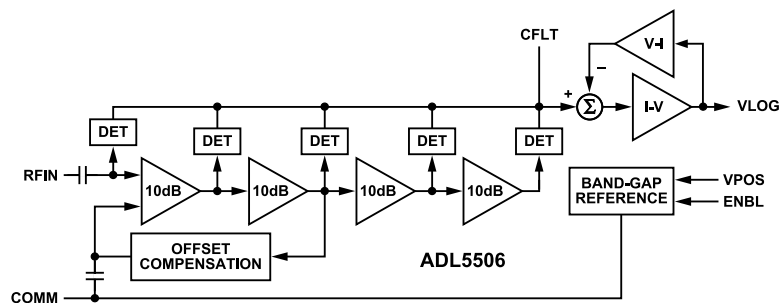
Figure 41. Block Schematic
