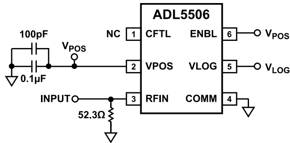
Figure 42. Basic Connections
