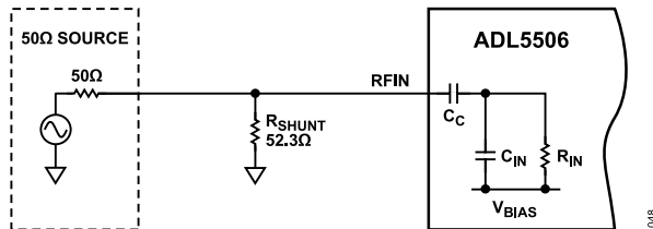
Figure 46. Broadband Resistive Method for Input Coupling
