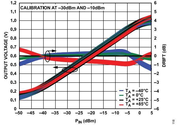
Figure 18. Distribution of Log Conformance Error with Respect to V_{LOG} at 25°C vs. P_{IN} and Temperature at 450 MHz
