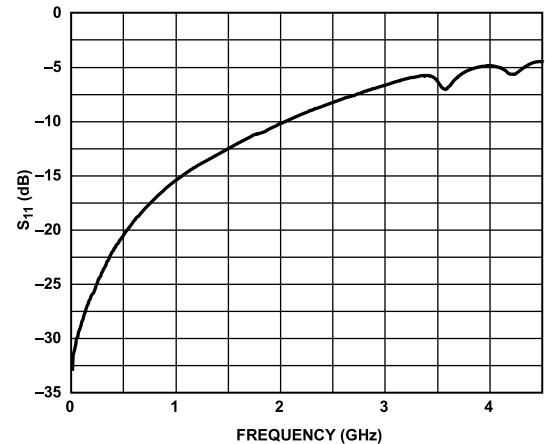
Figure 32. S_{11} at RF Input Port, 10 MHz to 4.5 GHz with 52.3 \Omega Shunt Resistor at RF Input Port
