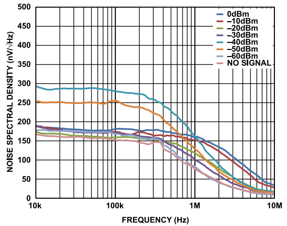
Figure 31. Noise Spectral Density, C_{FLT} = Open, 25°C
