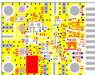
Figure 52. Layout of Evaluation Board, Component Side
