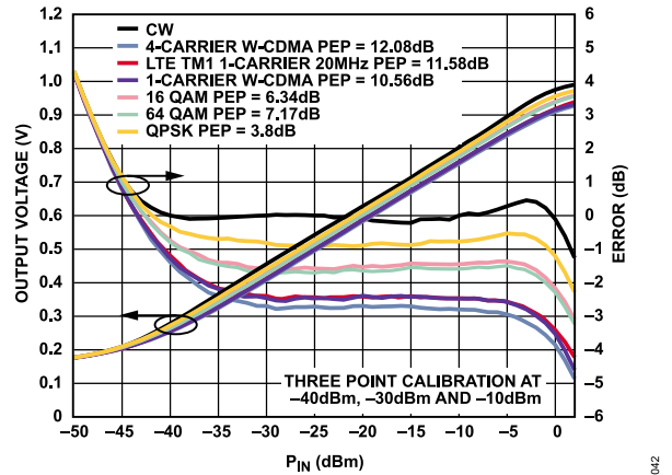
Figure 38. Error from CW Linear Reference vs. Signal Modulation (Four-Carrier W-CDMA, LTE TM1 One-Carrier 20 MHz, One-Carrier W-CDMA, 16 QAM, 64 QAM, QPSK), Frequency = 2.14 GHz
