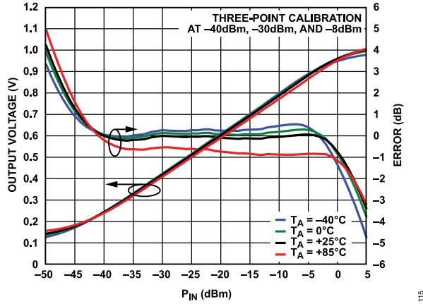
Figure 15. V_{LOG} and Log Conformance Error vs. P_{IN} over Temperature at 450 MHz
