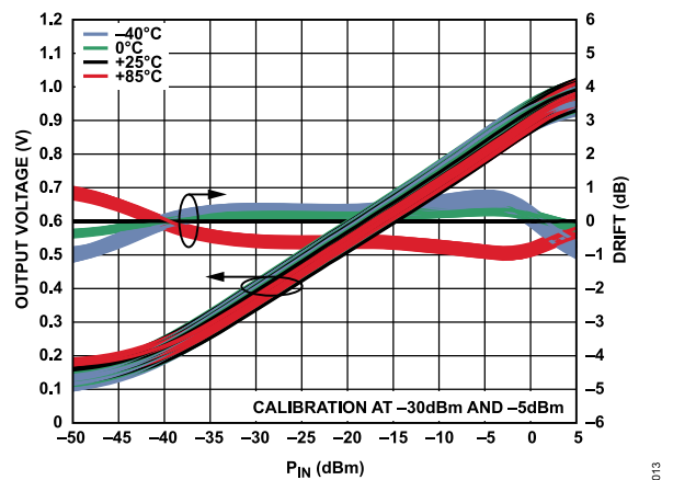
Figure 13. Distribution of Log Conformance Error with Respect to V_{LOG} at 25°C vs. P_{IN} and Temperature at 50 MHz
