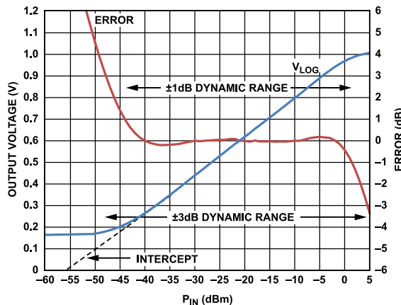
Figure 43. V LOG and Log Conformance Error vs. Input Level at 900 MHz
