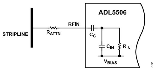
Figure 48. Series Attenuation Method for Input Coupling
