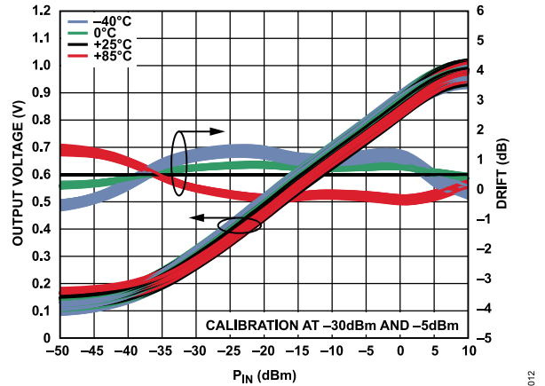
Figure 12. Distribution of Log Conformance Error with Respect to V_{LOG} at 25°C vs. P_{IN} and Temperature at 30 MHz
