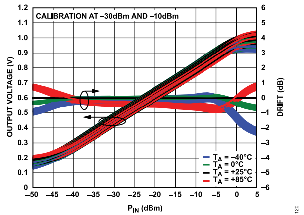
Figure 20. Distribution of Log Conformance Error with Respect to V_{LOG} at 25°C vs. P_{IN} and Temperature at 1900 MHz
