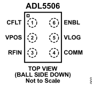
Figure 2. Pin Configuration
