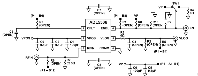
Figure 51. Evaluation Board Schematic
