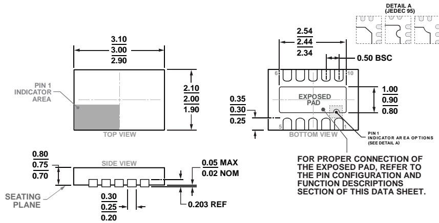
COMPLIANT TO JEDEC STANDARDS MO-229-WCED-3 Figure 69. 10-Lead Lead Frame Chip Scale Package [LFCSPP] 3 mm x 2 mm Body and 0.75 mm Package Height (CP-10-12) Dimensions shown in millimeters
