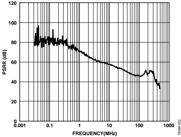
Figure 52. Power Supply Rejection Ratio (PSRR) vs. Frequency, 200 mV p-p at the VPOS Pin (See Figure 58 for the PSRR Measurement Setup)
