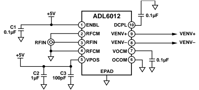
Figure 59. Basic Connections
