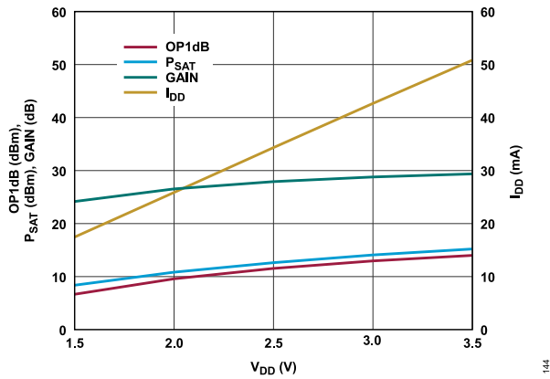
Figure 44. OP1dB, P_{SAT} , Gain, and I_{DD} vs. Supply Voltage at 31 GHz, R_{BIAS} = 634 \Omega
