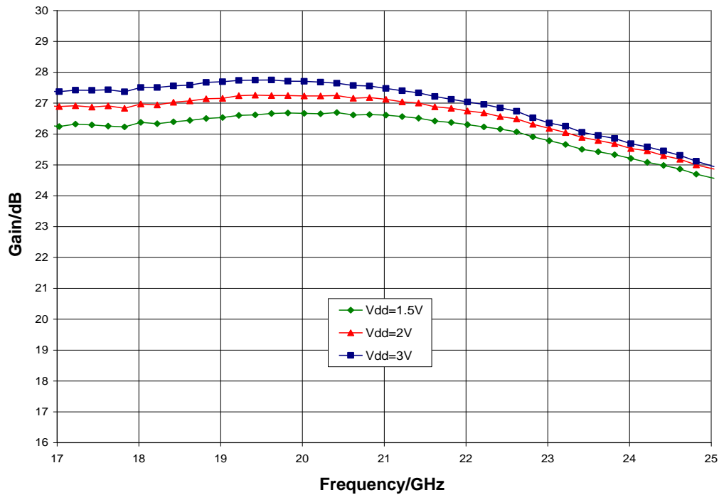
Gain vs. V_{dd} , V_{gg} = 1.5\text{ V} , T_A = 25\text{ }^\circ\text{C}
