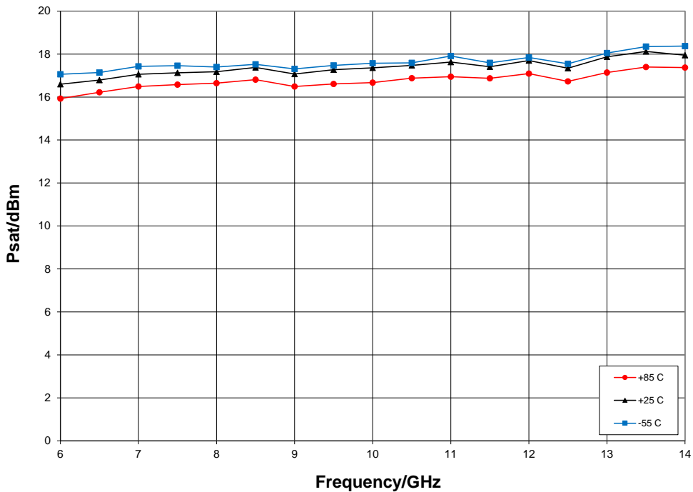
Psat vs. Temperature, V_{dd} = 3\text{ V} , V_{gg} = 1.5\text{ V}
