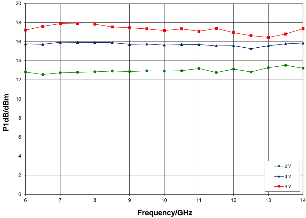
P1dB vs. V_{dd} , V_{gg} = 1.5\text{ V} , T_A = 25\text{ }^\circ\text{C}
