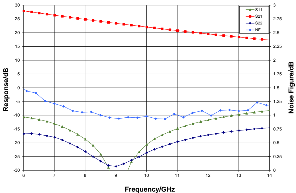
Narrow-band Performance, V_{dd} = 3\text{ V} , V_{gg} = 1.5\text{ V} , T_A = 25\text{ }^\circ\text{C}
