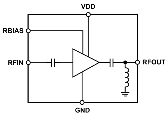
Figure 48. Simplified Schematic
